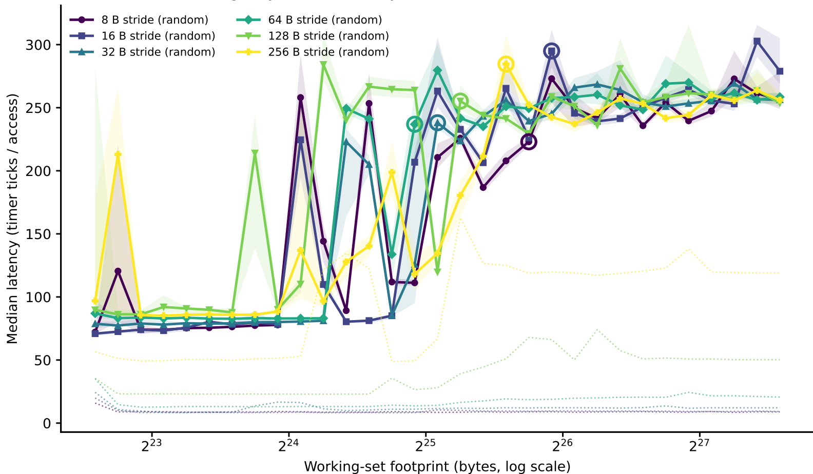
hazel_icelake_8358: line-size family of curves (dependent pointer chase) (Phase I timing-only, level boundary=50331648B window=[6291456,201326592])
