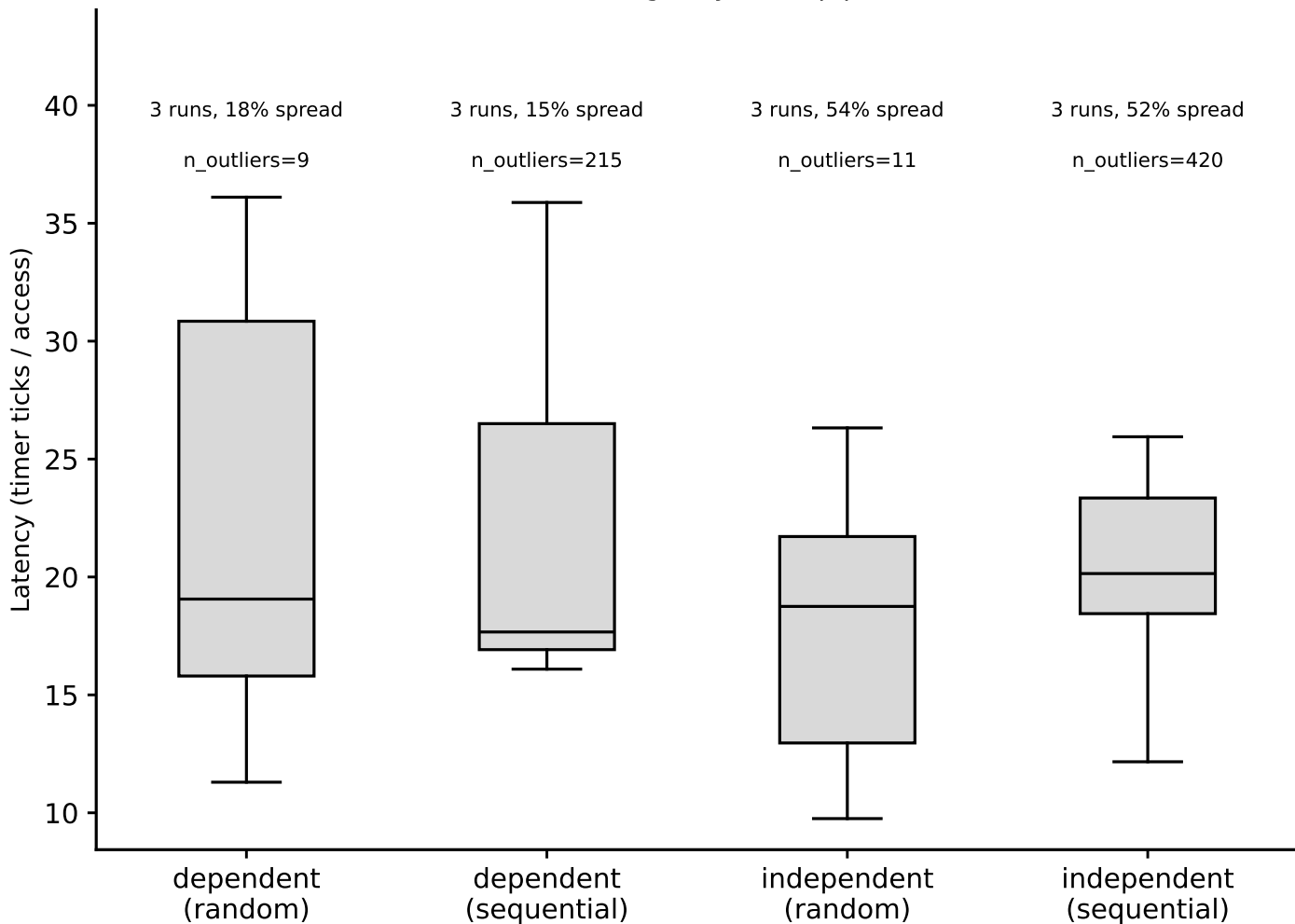
hazel_sapphirerapids: hit-latency box plots, L1 (footprint=48 KiB) (Phase I timing-only, auto pipeline)
