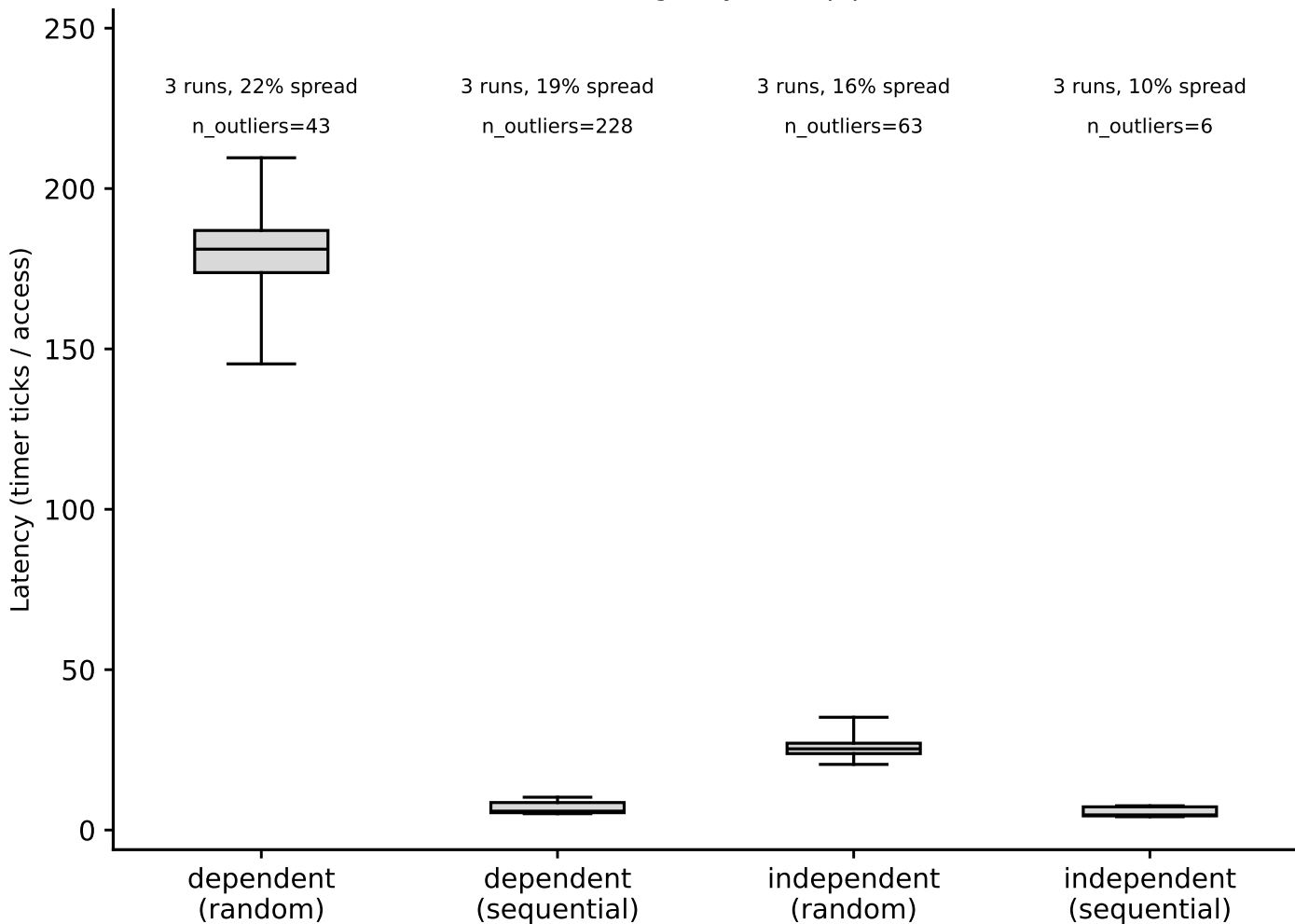
hazel_sapphirerapids: hit-latency box plots, LLC (footprint=38.0546 MiB) (Phase I timing-only, auto pipeline)
