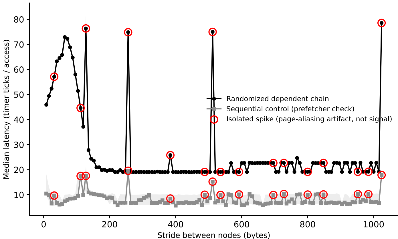
hazel_sapphirerapids: line-size sweep (dependent pointer chase), footprint=4 MiB (Phase I timing-only, level boundary=2097152B, single-curve method)
