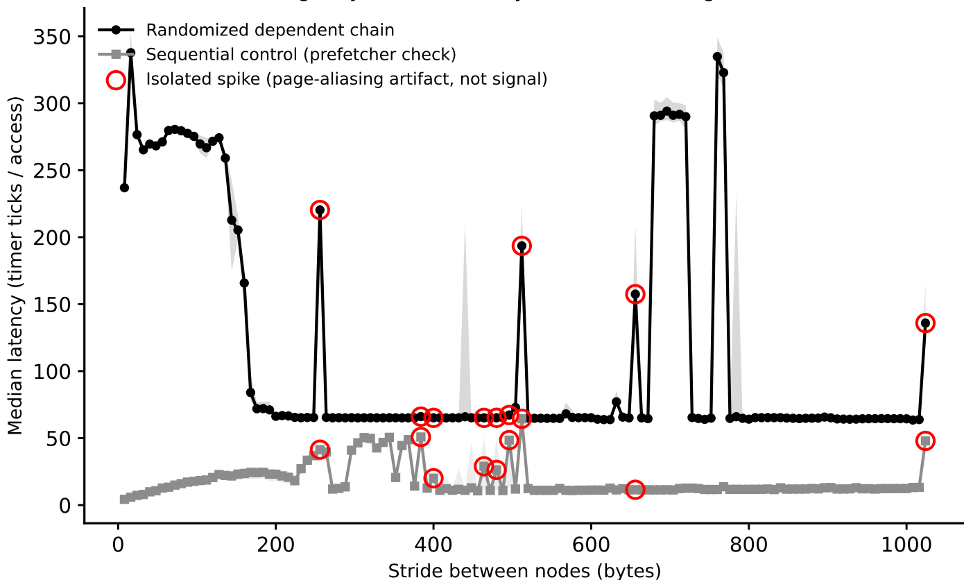
hazel_sapphirerapids: line-size sweep (dependent pointer chase), footprint=76.1093 MiB (Phase I timing-only, level boundary=39903168B, single-curve method)
