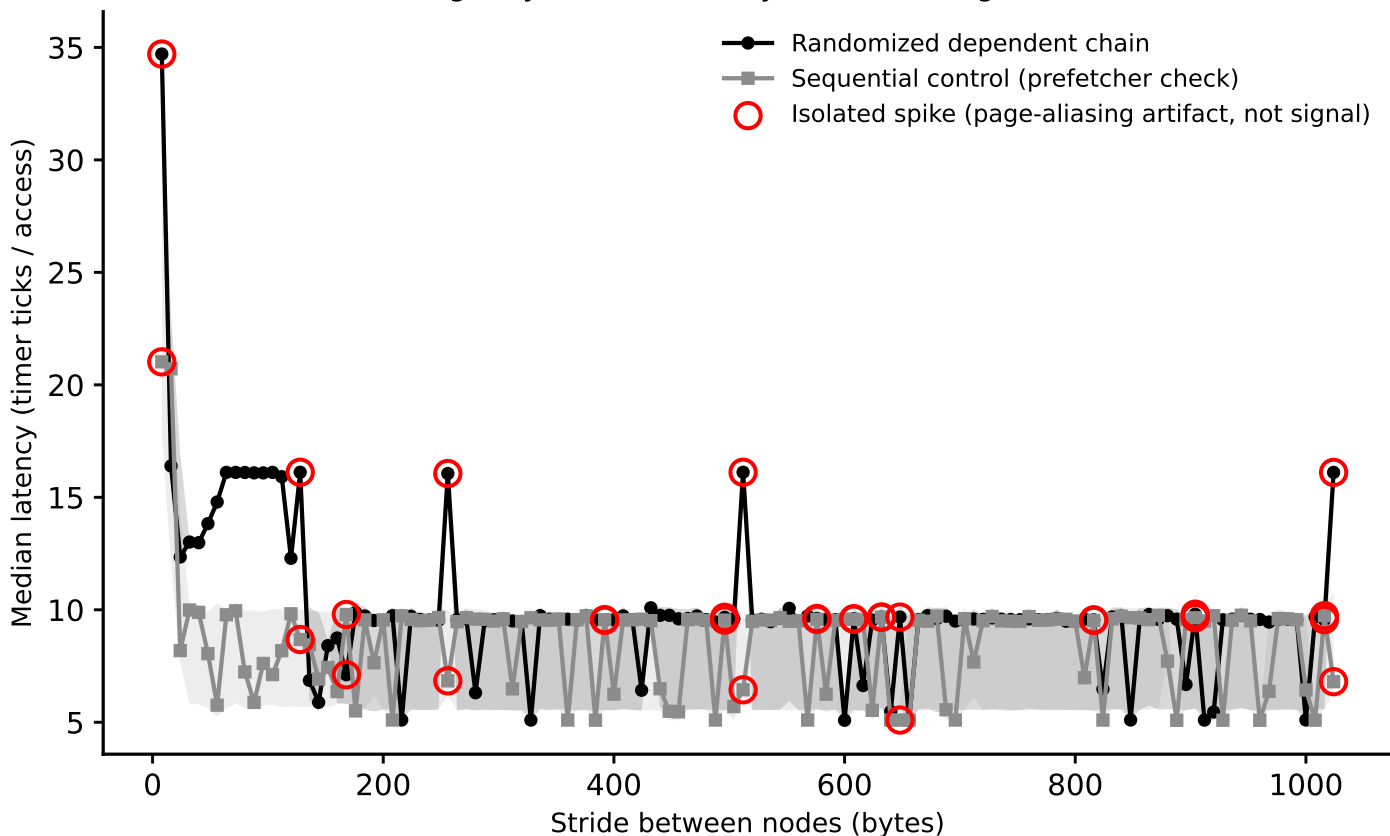
hazel_sapphirerapids: line-size sweep (dependent pointer chase), footprint=96 KiB (Phase I timing-only, level boundary=49152B, single-curve method)
