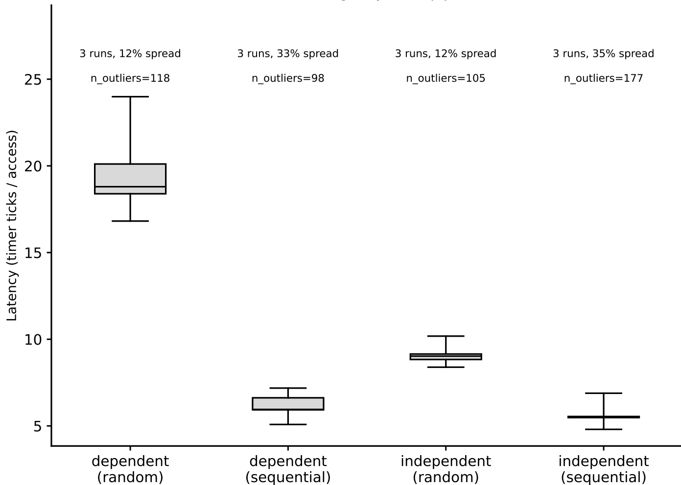
hazel_skylake: hit-latency box plots, L2 (footprint=1 MiB) (Phase I timing-only, auto pipeline)
