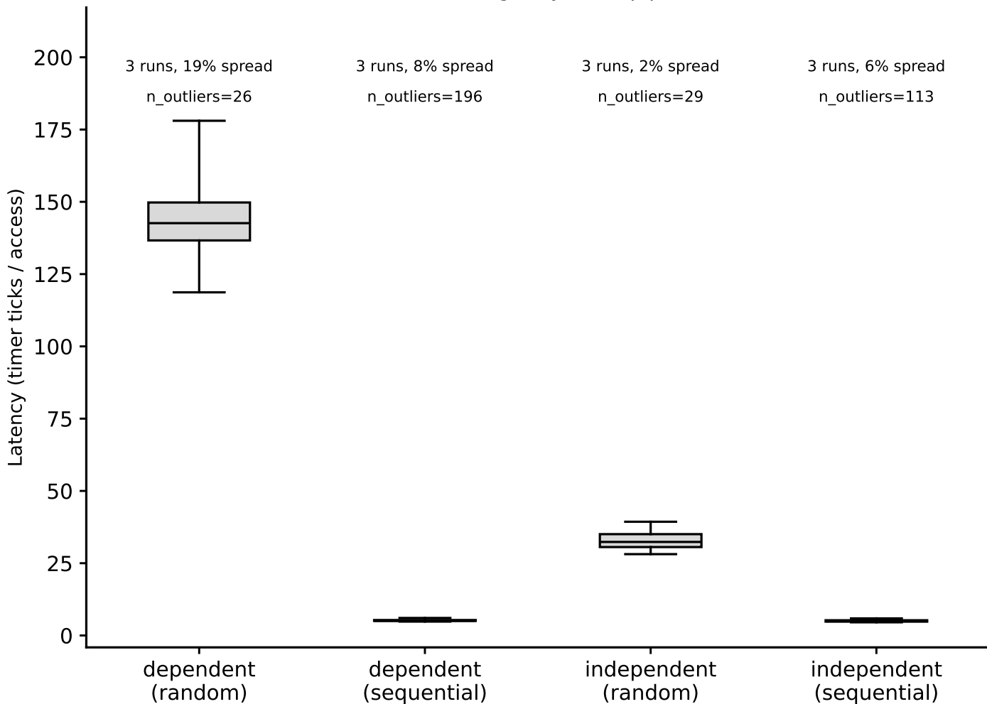
hazel_skylake: hit-latency box plots, LLC (footprint=22.6274 MiB) (Phase I timing-only, auto pipeline)
