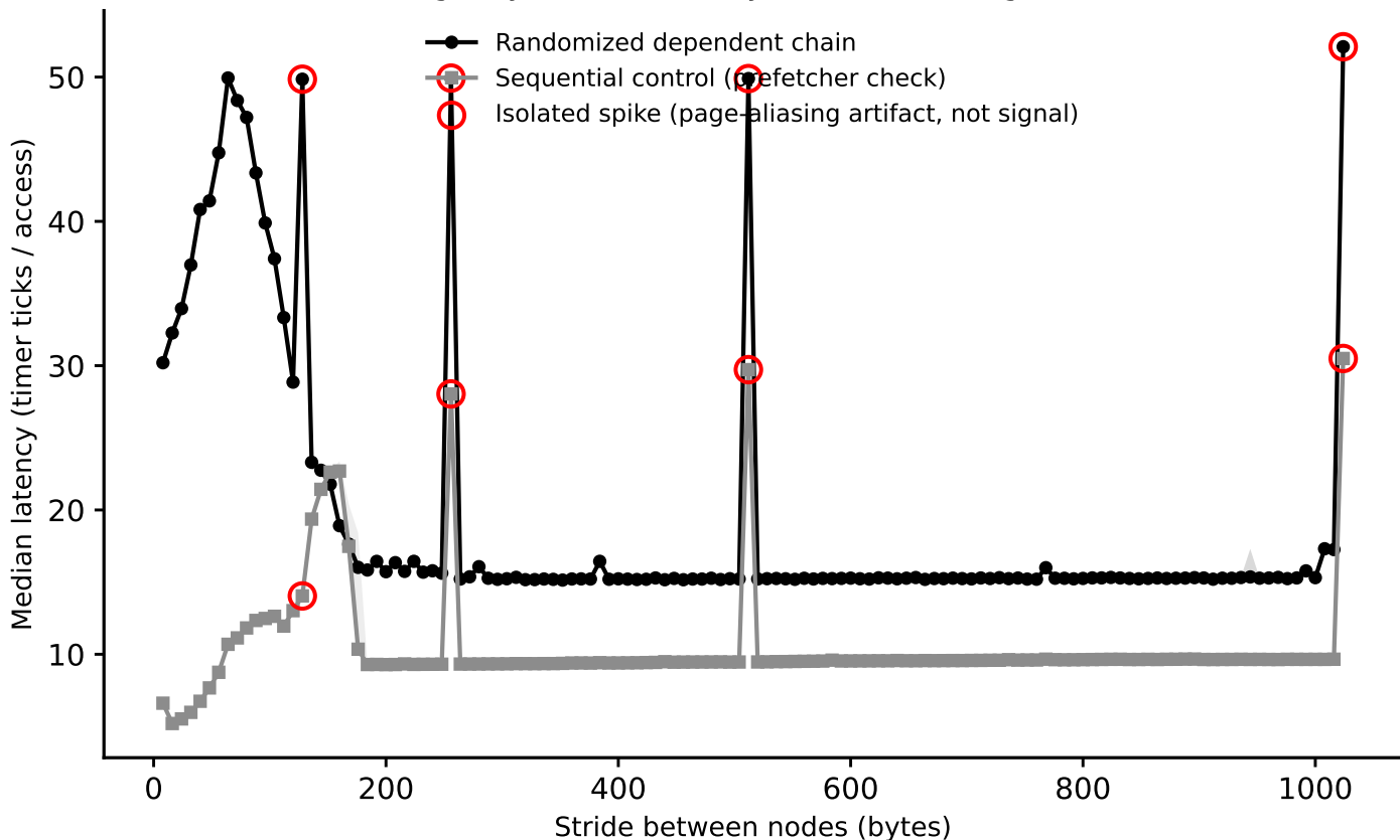
hazel_skylake: line-size sweep (dependent pointer chase), footprint=2 MiB (Phase I timing-only, level boundary=1048576B, single-curve method)
