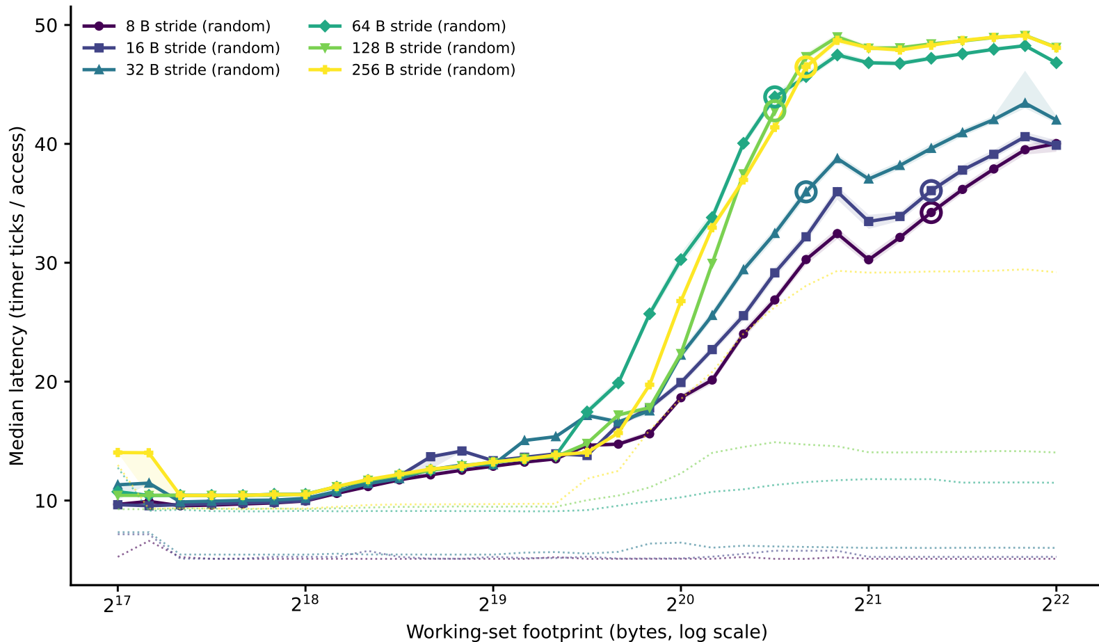
hazel_skylake: line-size family of curves (dependent pointer chase) (Phase I timing-only, level boundary=1048576B window=[131072,4194304])
