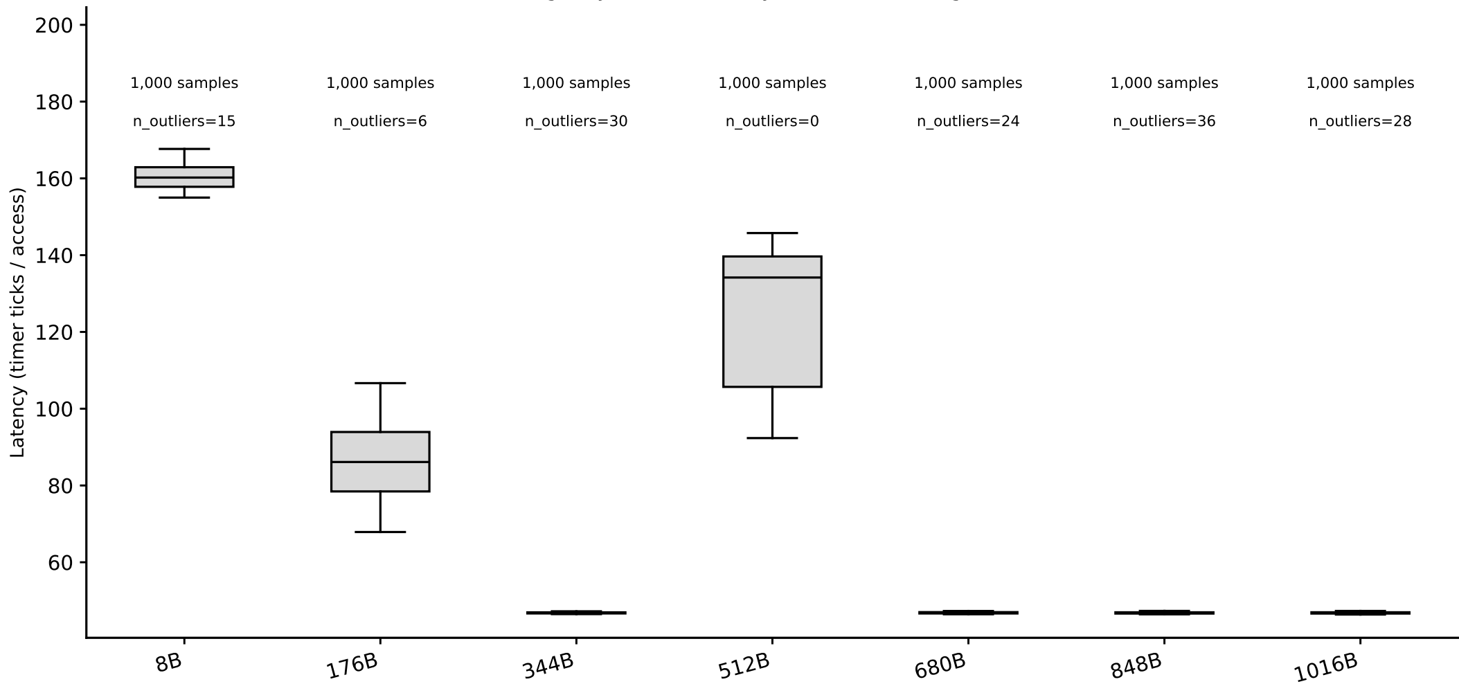
hazel_skylake: line-size box plots, random pattern (whiskers = p5/p95) (Phase I timing-only, level boundary=23726560B, single-curve method)
