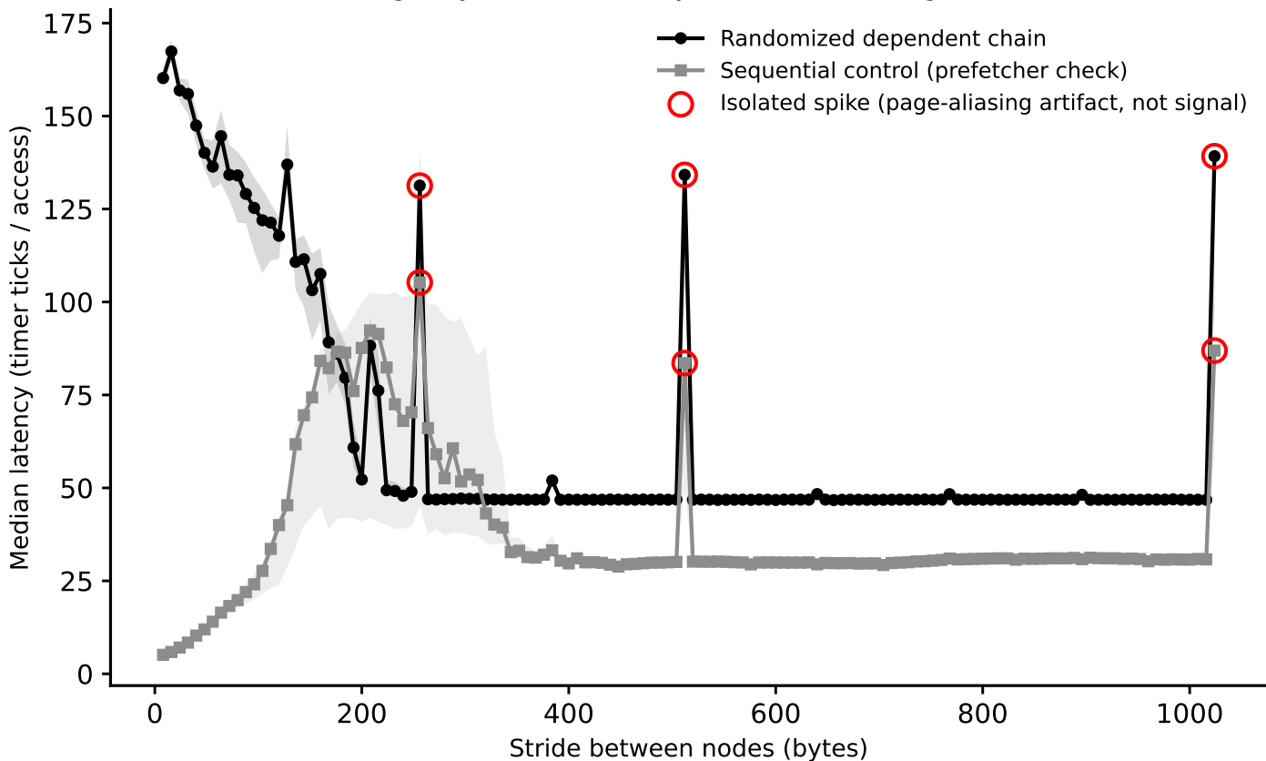
hazel_skylake: line-size sweep (dependent pointer chase), footprint=45.2548 MiB (Phase I timing-only, level boundary=23726560B, single-curve method)
