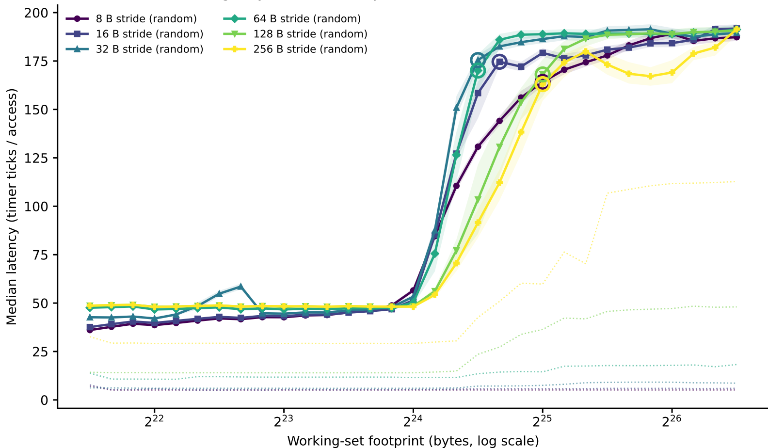
hazel_skylake: line-size family of curves (dependent pointer chase) (Phase I timing-only, level boundary=23726560B window=[2965820,94906240])
