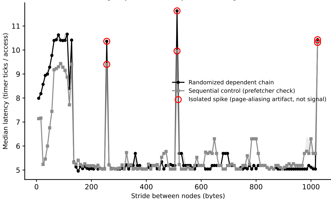
hazel_skylake: line-size sweep (dependent pointer chase), footprint=64 KiB (Phase I timing-only, level boundary=32768B, single-curve method)
