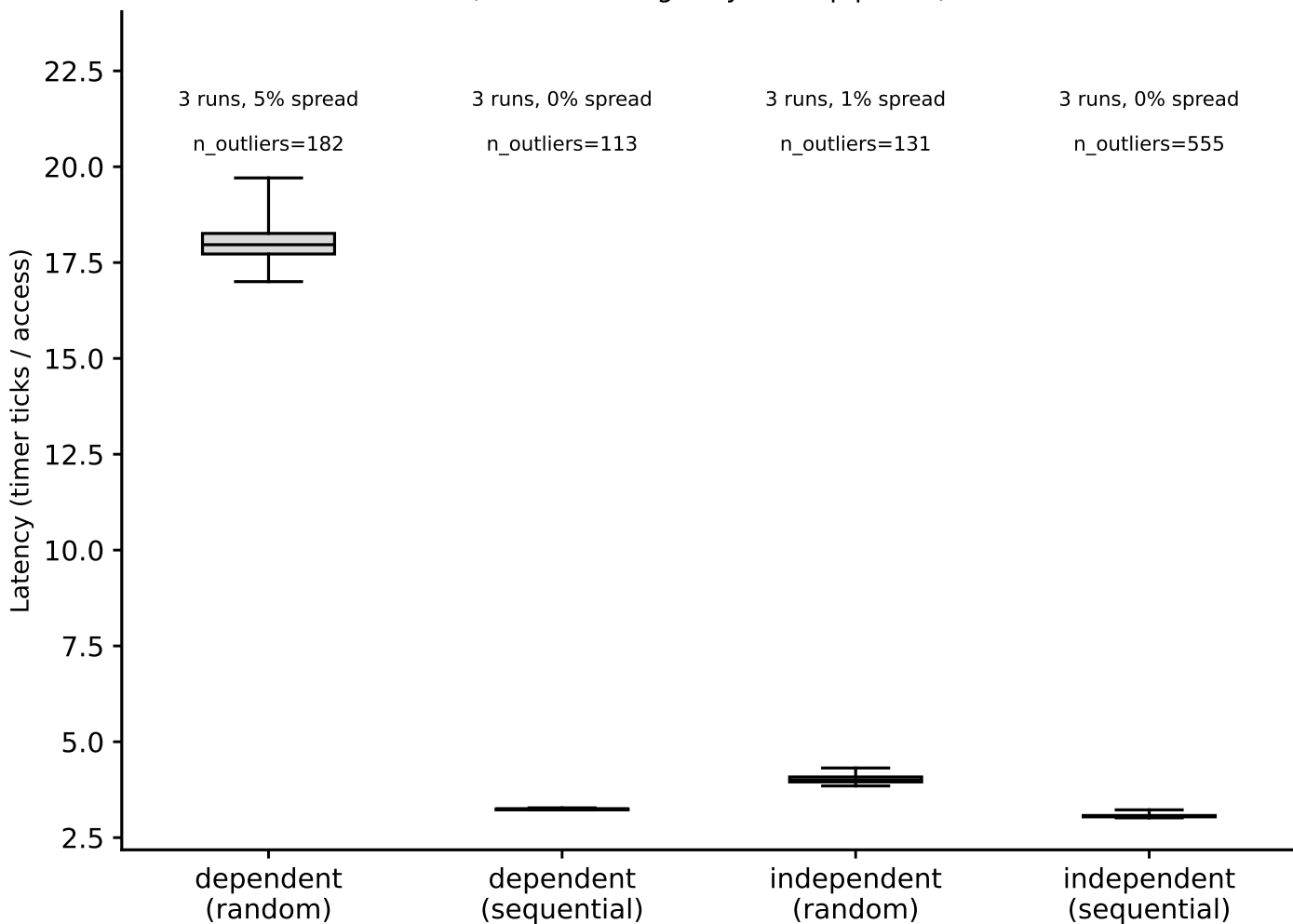
hazel_turin: hit-latency box plots, L2 (footprint=1 MiB) (Phase I timing-only, auto pipeline)
