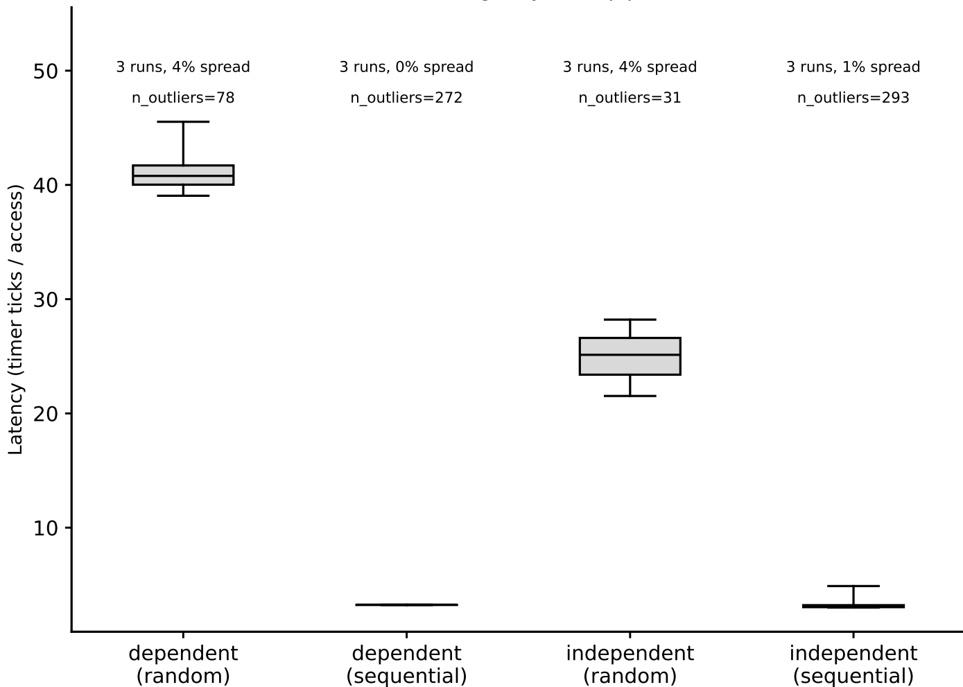
hazel_turin: hit-latency box plots, LLC (footprint=32 MiB) (Phase I timing-only, auto pipeline)
