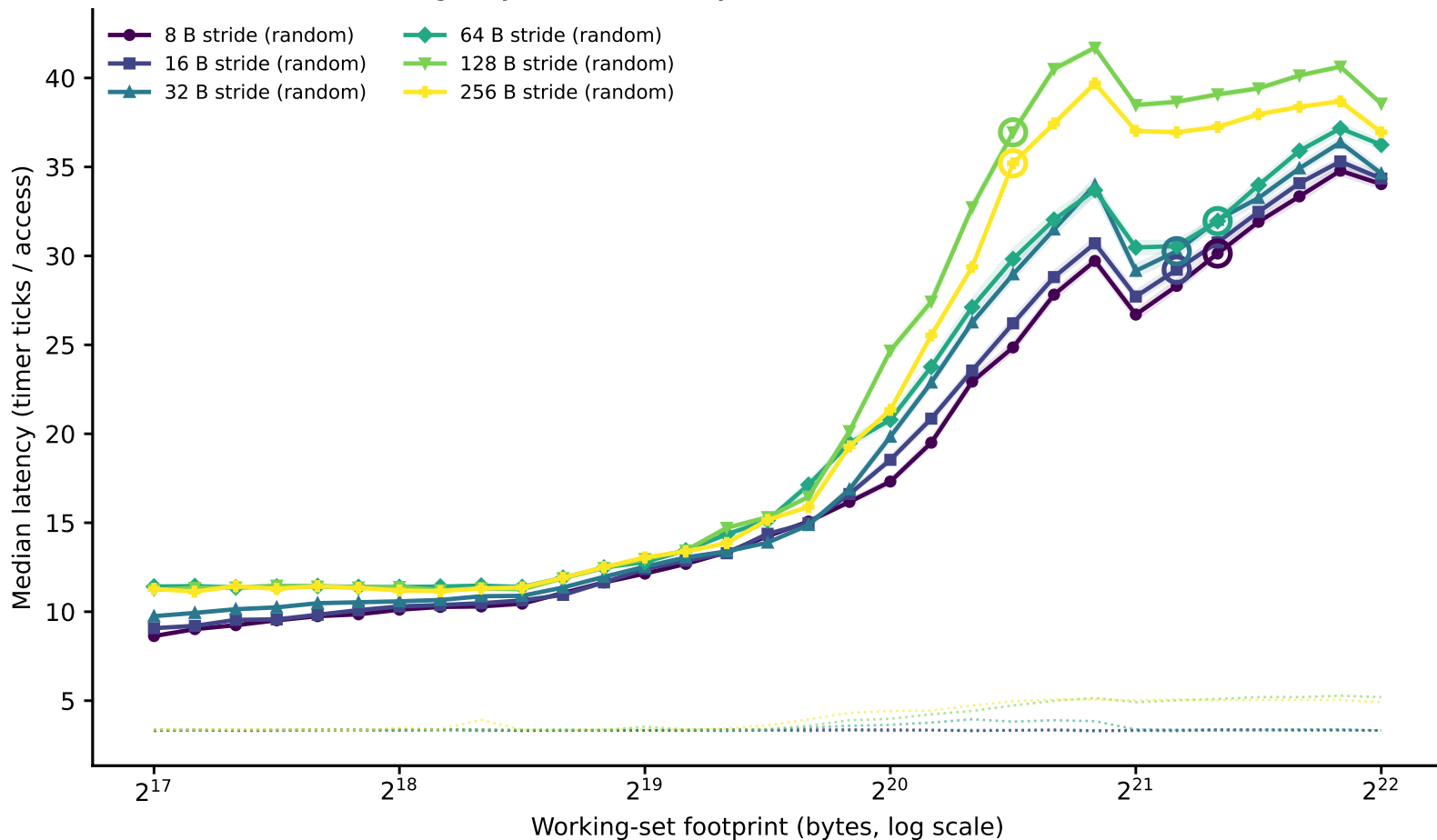
hazel_turin: line-size family of curves (dependent pointer chase) (Phase I timing-only, level boundary=1048576B window=[131072,4194304])
