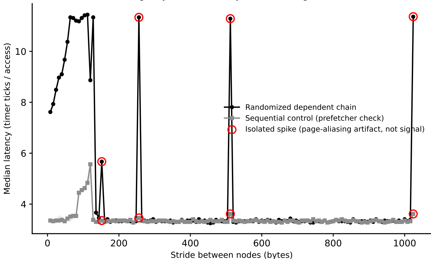
hazel_turin: line-size sweep (dependent pointer chase), footprint=96 KiB (Phase I timing-only, level boundary=49152B, single-curve method)
