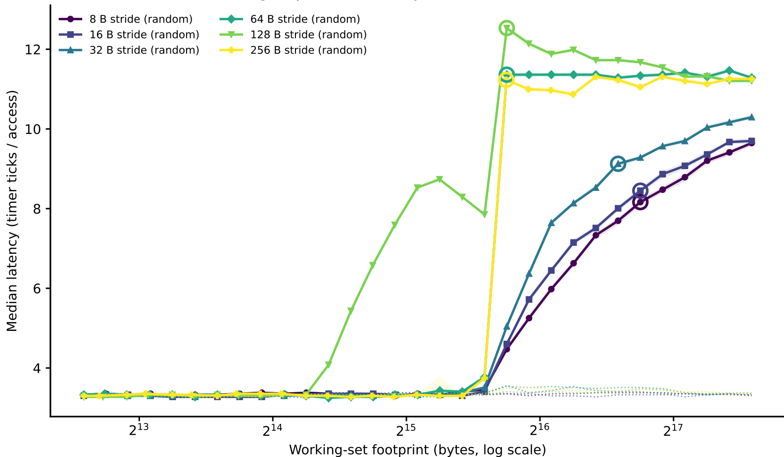
hazel_turin: line-size family of curves (dependent pointer chase) (Phase I timing-only, level boundary=49152B window=[6144,196608])
