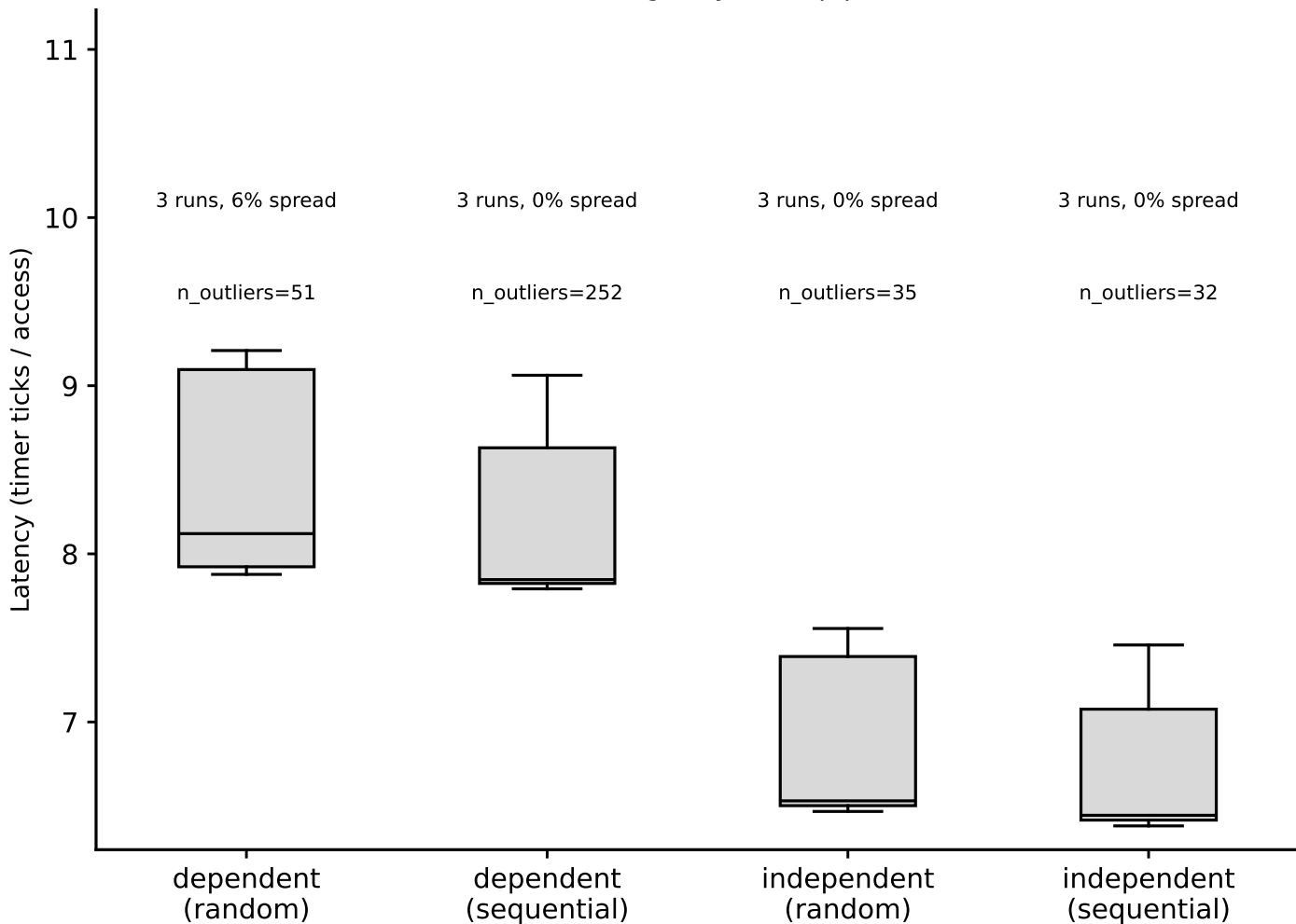
hazel_haswell: hit-latency box plots, L1 (footprint=32 KiB) (Phase I timing-only, auto pipeline)
