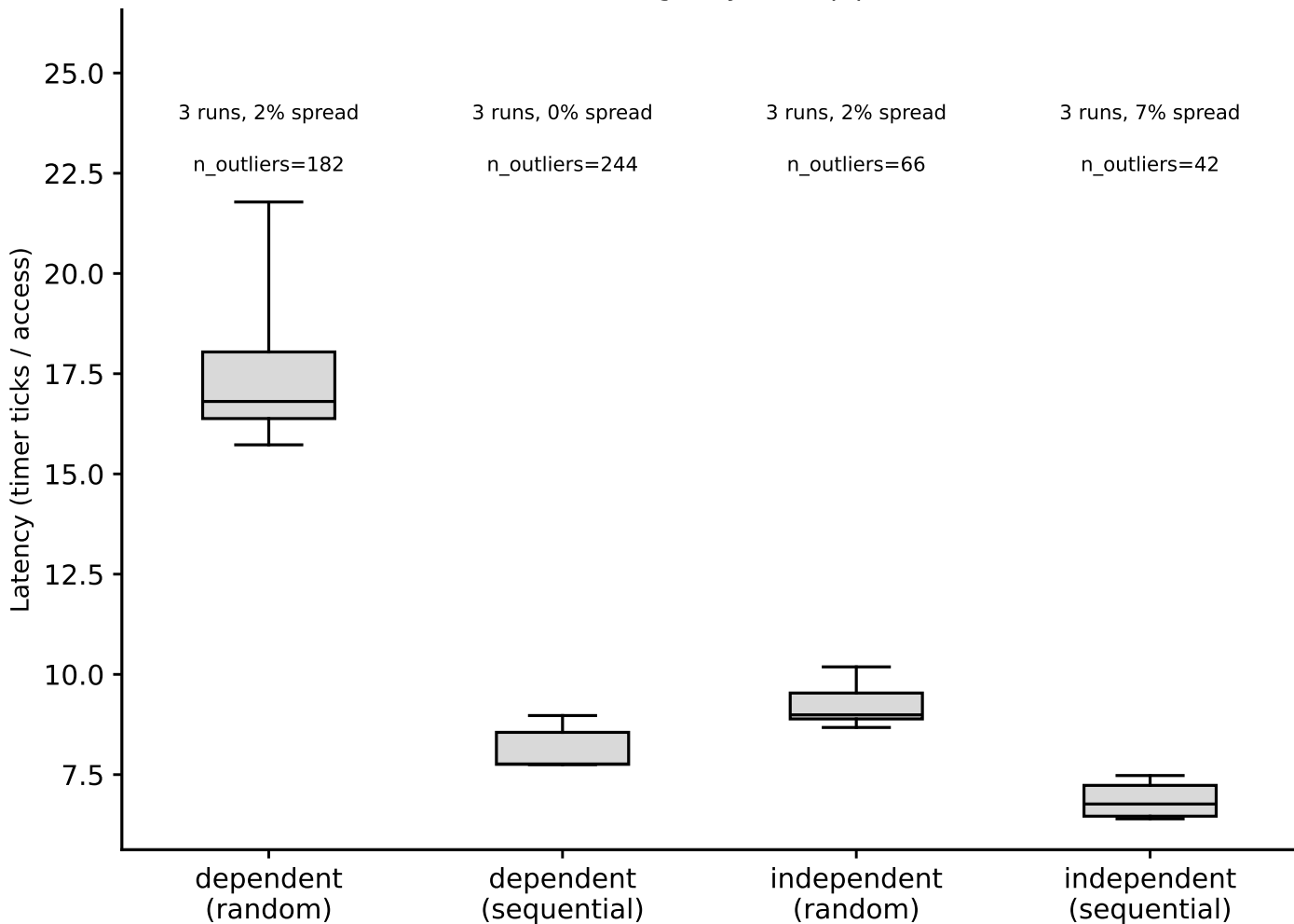
hazel_haswell: hit-latency box plots, L2 (footprint=256 KiB) (Phase I timing-only, auto pipeline)
