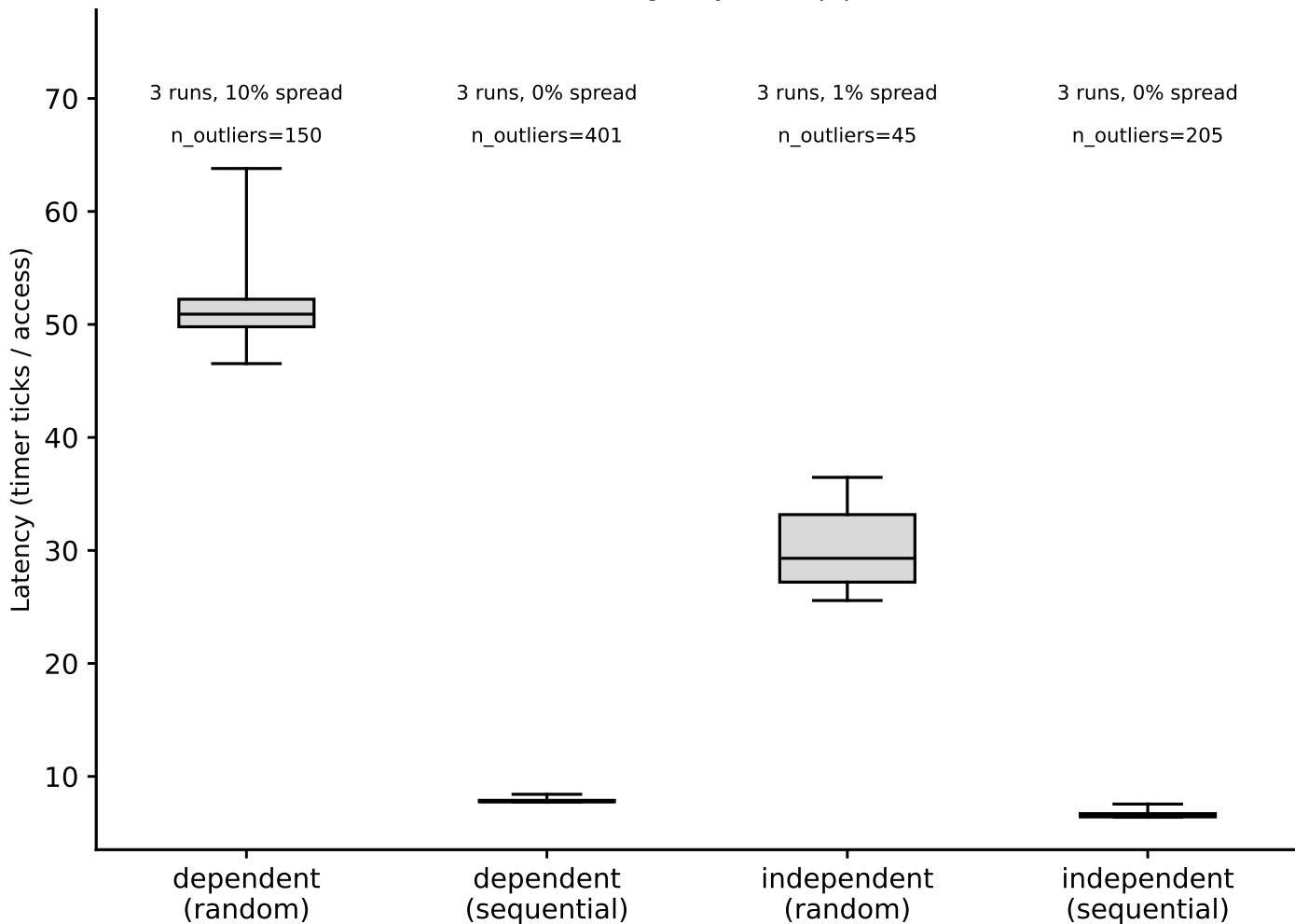
hazel_haswell: hit-latency box plots, LLC (footprint=24 MiB) (Phase I timing-only, auto pipeline)
