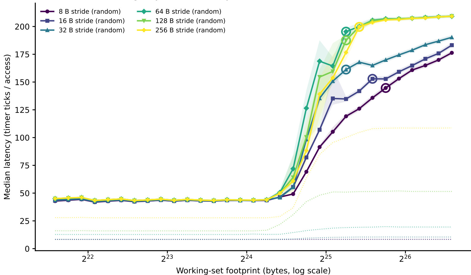
hazel_haswell: line-size family of curves (dependent pointer chase) (Phase I timing-only, level boundary=25165824B window=[3145728,100663296])
