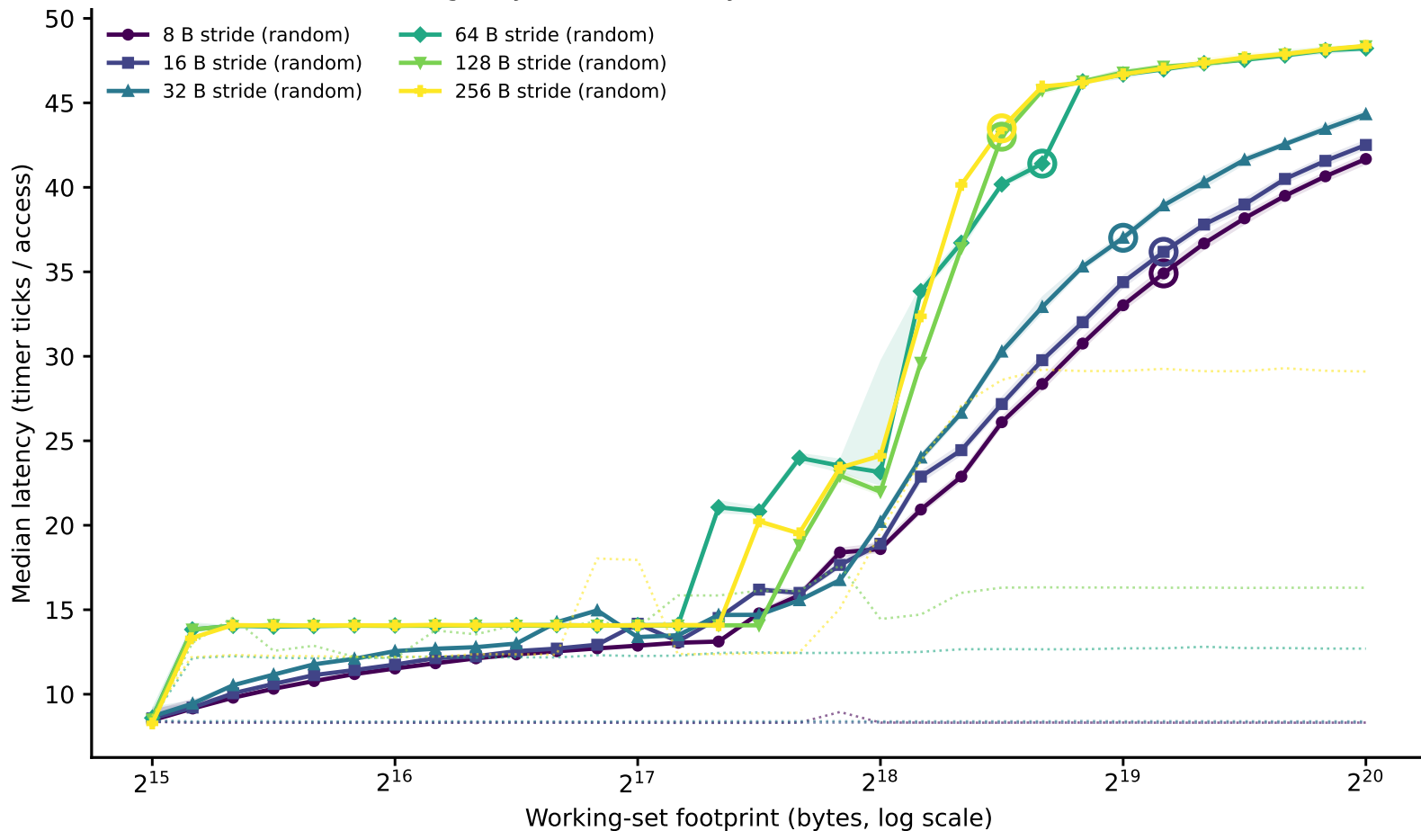
hazel_haswell: line-size family of curves (dependent pointer chase) (Phase I timing-only, level boundary=262144B window=[32768,1048576])
