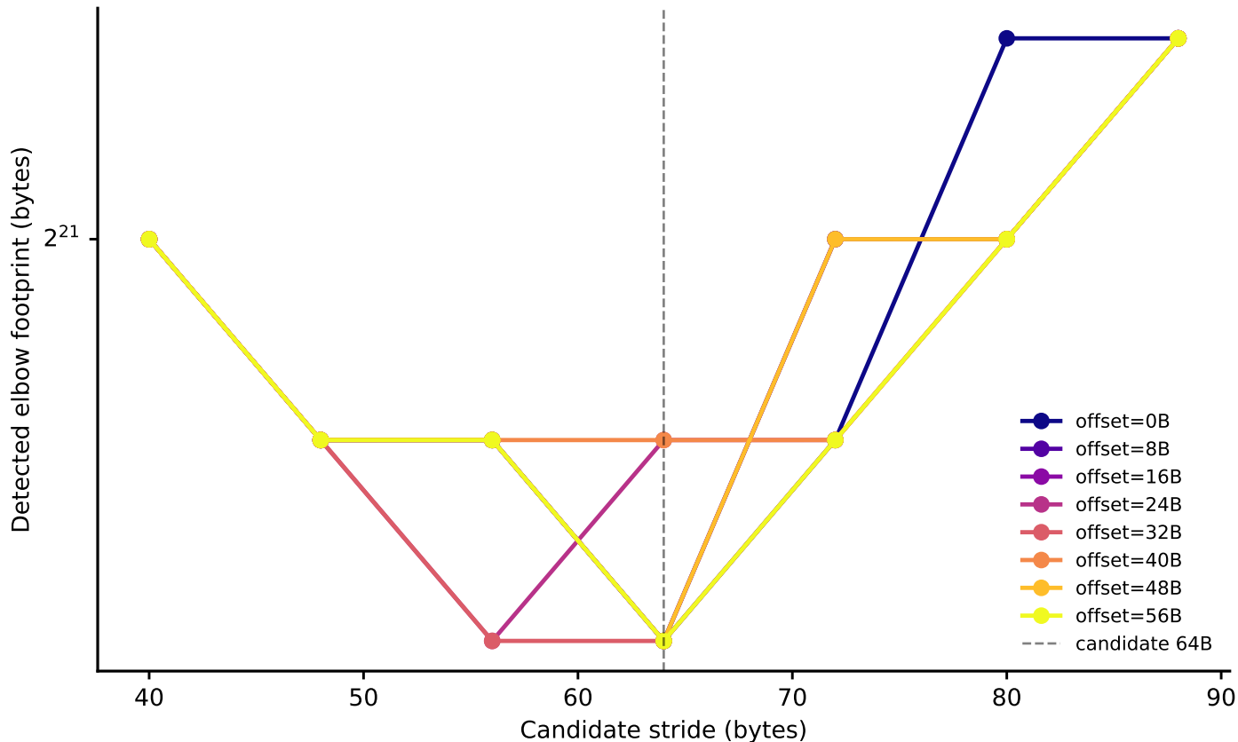
thunderbird: line-size elbow vs. stride, by node-0 offset (Phase I timing-only, level boundary=1048576B, step-4 alignment refinement)
