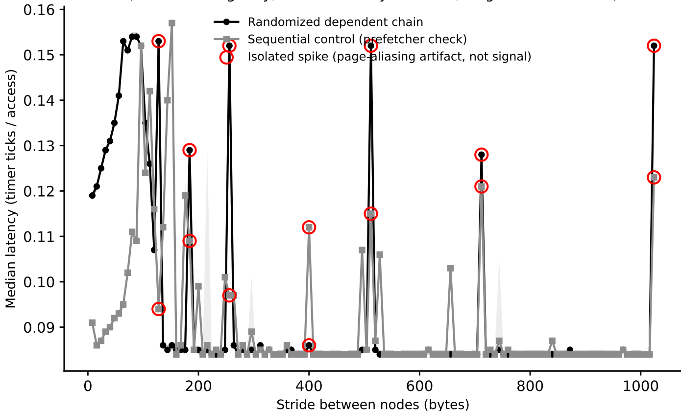
thunderbird: line-size sweep (dependent pointer chase), footprint=128 KiB (Phase I timing-only, level boundary=65536B, single-curve method)
