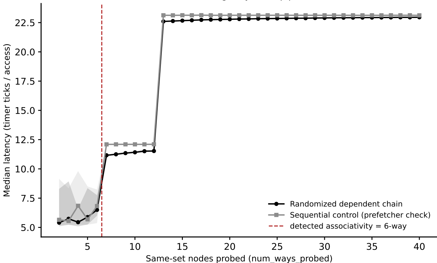
artemisia: associativity sweep, L2 (stride=2 MiB) (Phase I timing-only, auto pipeline)
