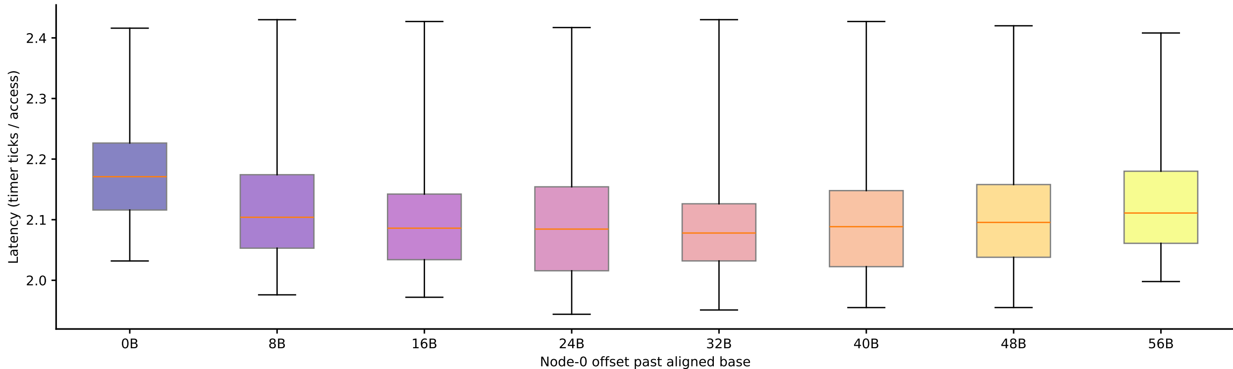
thunderbird: candidate stride 128 B at footprint 53.4539 MiB, by offset (Phase I timing-only, level boundary=31457280B, step-4 repro repeat seed=12346, compare vs seed=12345)
