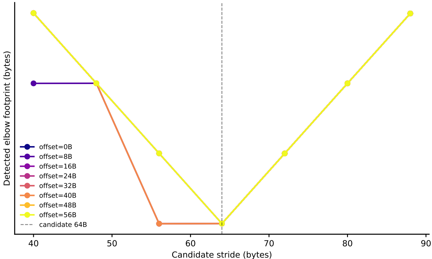
thunderbird: line-size elbow vs. stride, by node-0 offset (Phase I timing-only, level boundary=65536B, step-4 alignment refinement)
