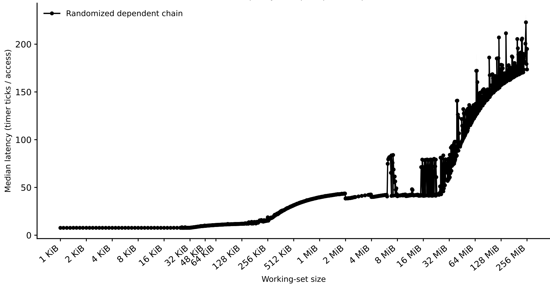
Hazel-Broadwell: capacity sweep (dependent pointer chase)
