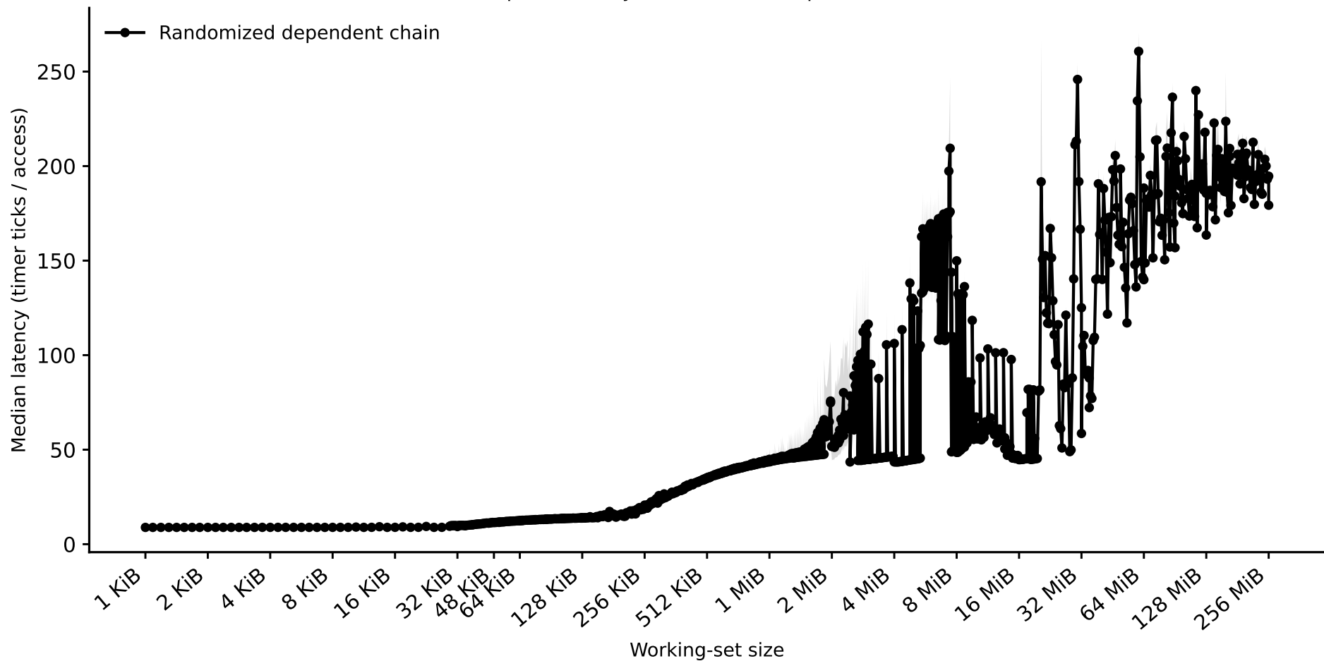
Hazel-Broadwell: capacity sweep (dependent pointer chase) (2026-09-15 reproducibility re-run -- uninterpreted, see CLAUDE.md)
