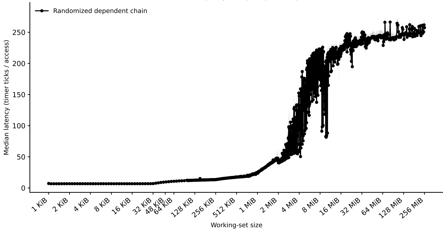
Hazel-Cascadelake: capacity sweep (dependent pointer chase)
