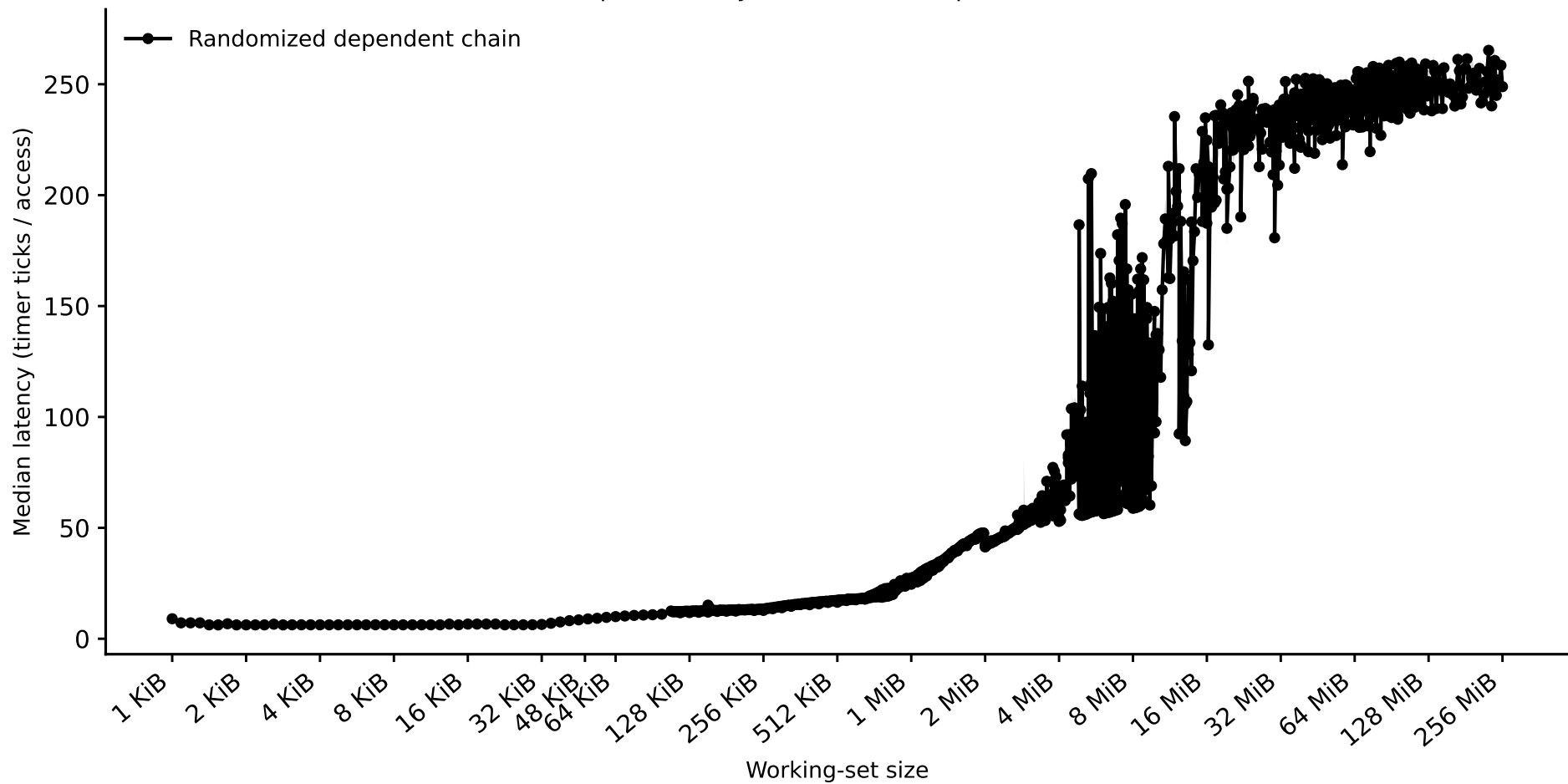
Hazel-Cascadelake: capacity sweep (dependent pointer chase) (2026-09-15 reproducibility re-run -- uninterpreted, see CLAUDE.md)
