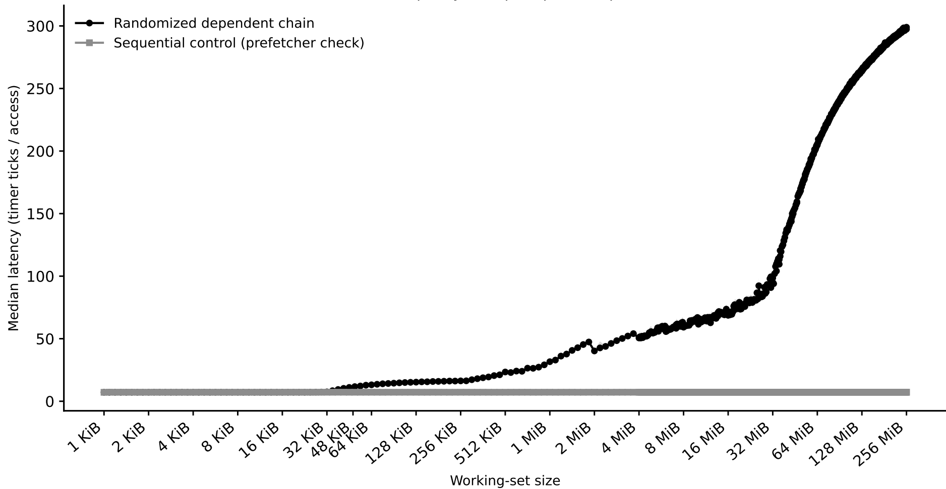
Hazel-Genoa: capacity sweep (dependent pointer chase)
