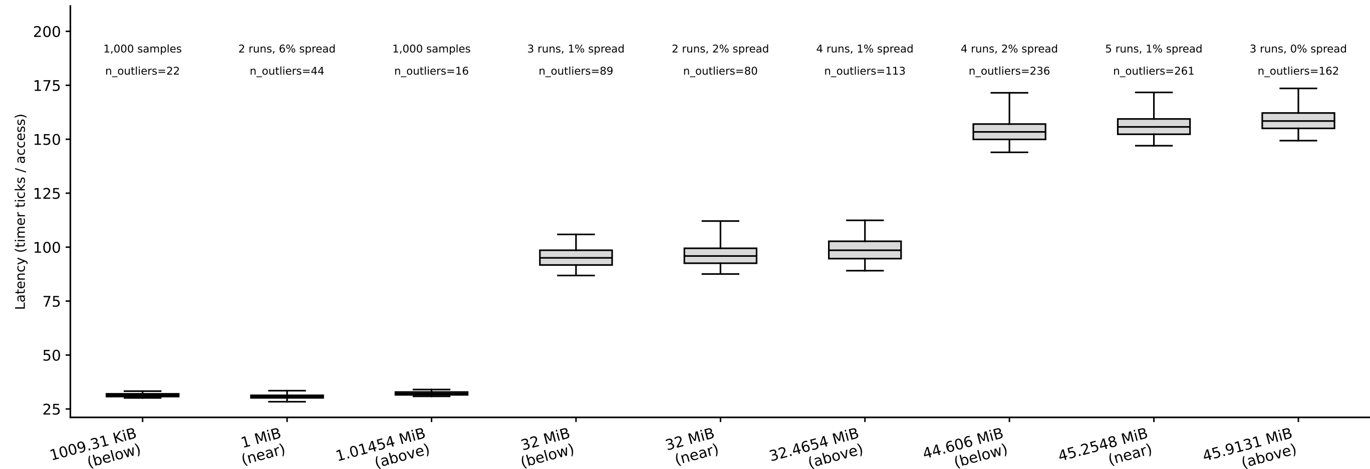
hazel_genoa/capacity_rerun: capacity box plots, random pattern (whiskers = p5/p95) (Phase I timing-only, auto pipeline) tested boundaries: 1 MiB, 32 MiB, 45.2548 MiB
