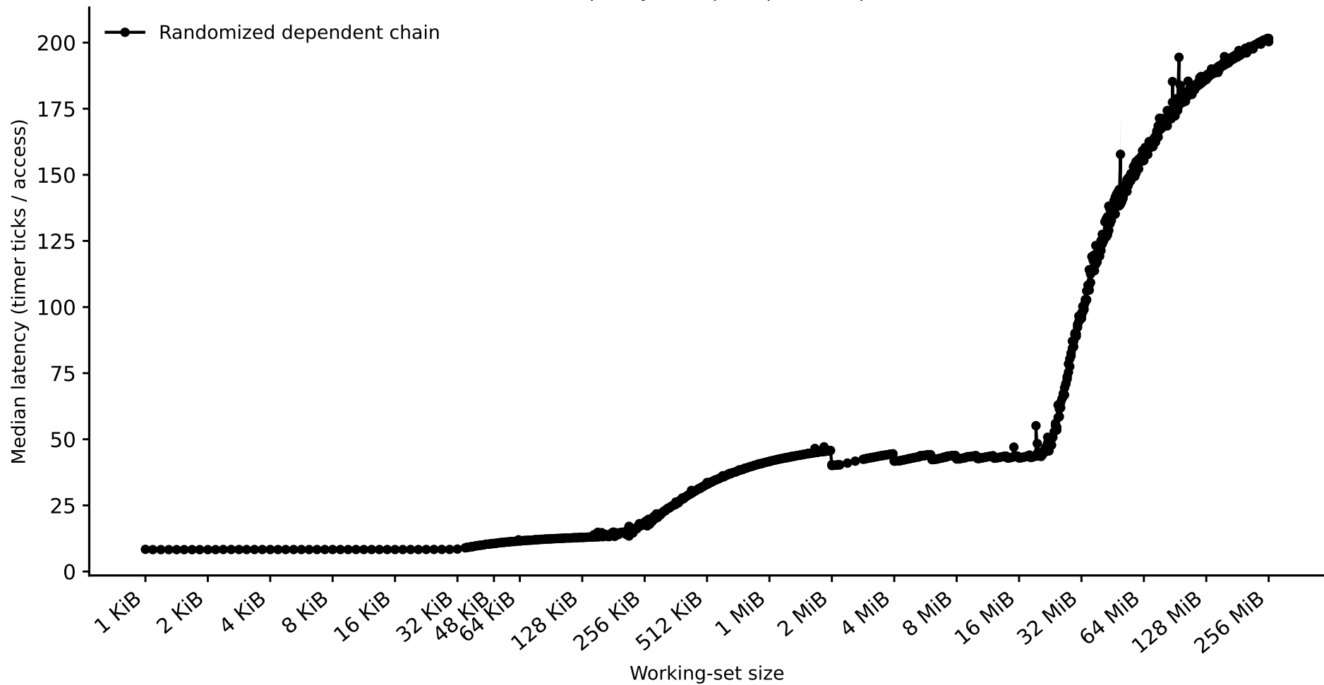
Hazel-Haswell: capacity sweep (dependent pointer chase)
