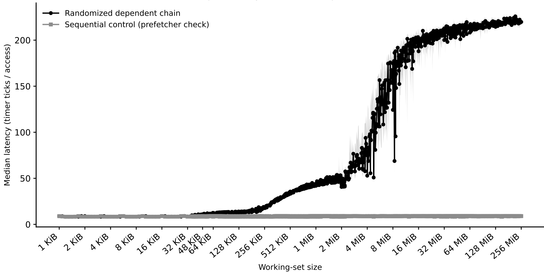
Hazel-Haswell: capacity sweep (dependent pointer chase) (2026-09-15 reproducibility re-run -- uninterpreted, see CLAUDE.md)
