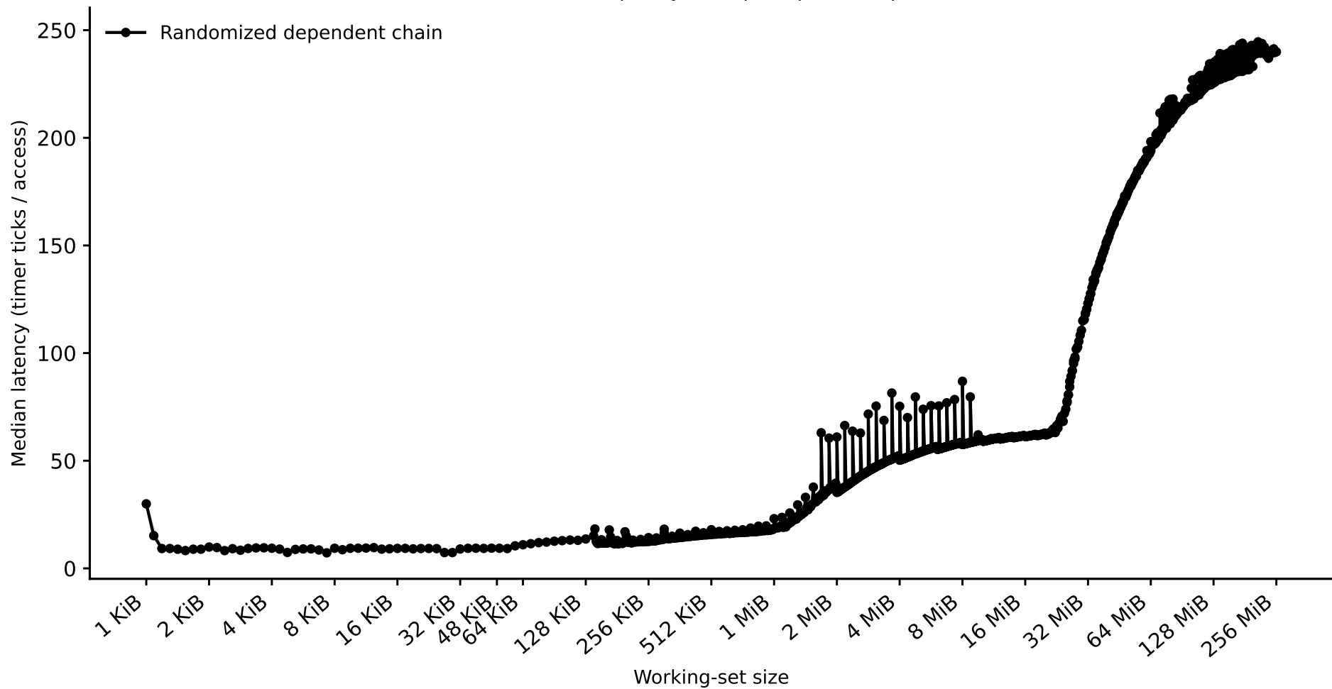
Hazel-Icelake-6326: capacity sweep (dependent pointer chase)
