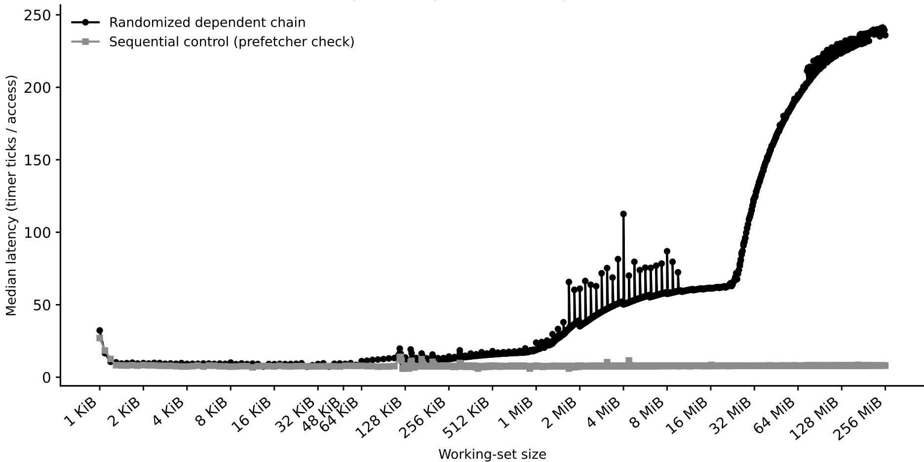
Hazel-Icelake-6326: capacity sweep (dependent pointer chase) (2026-09-15 reproducibility re-run -- uninterpreted, see CLAUDE.md)
