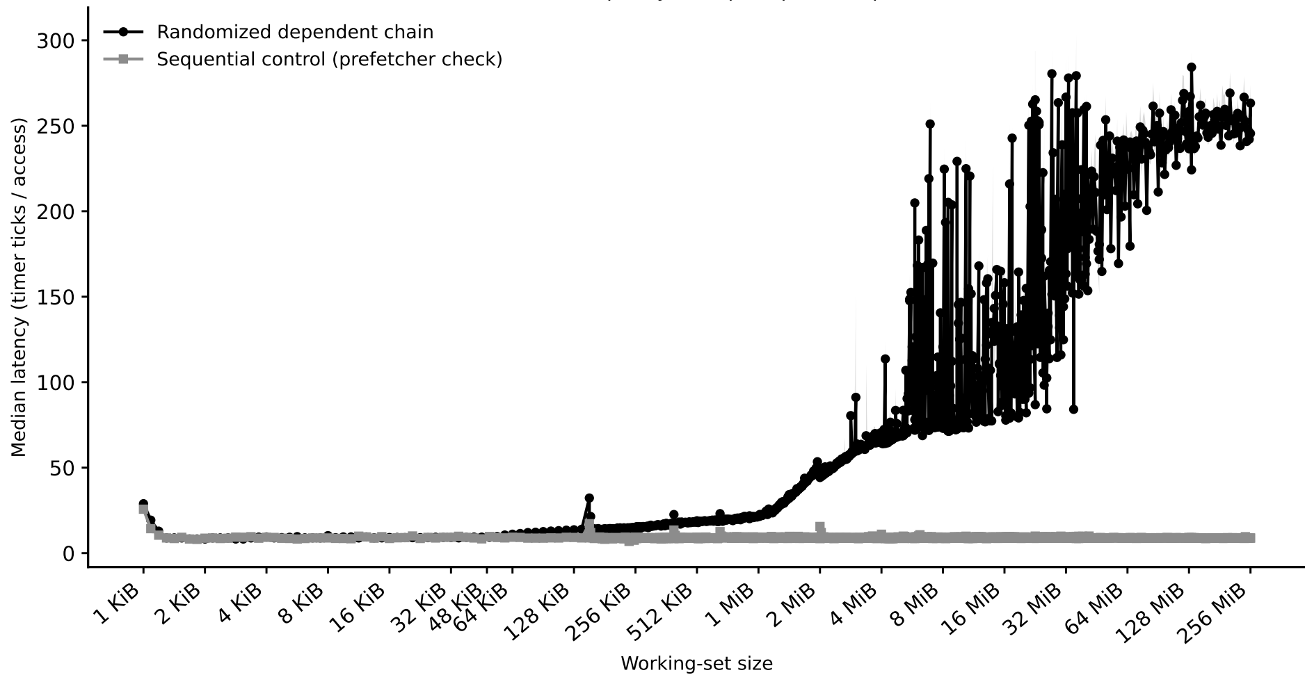
Hazel-Icelake-8358: capacity sweep (dependent pointer chase)
