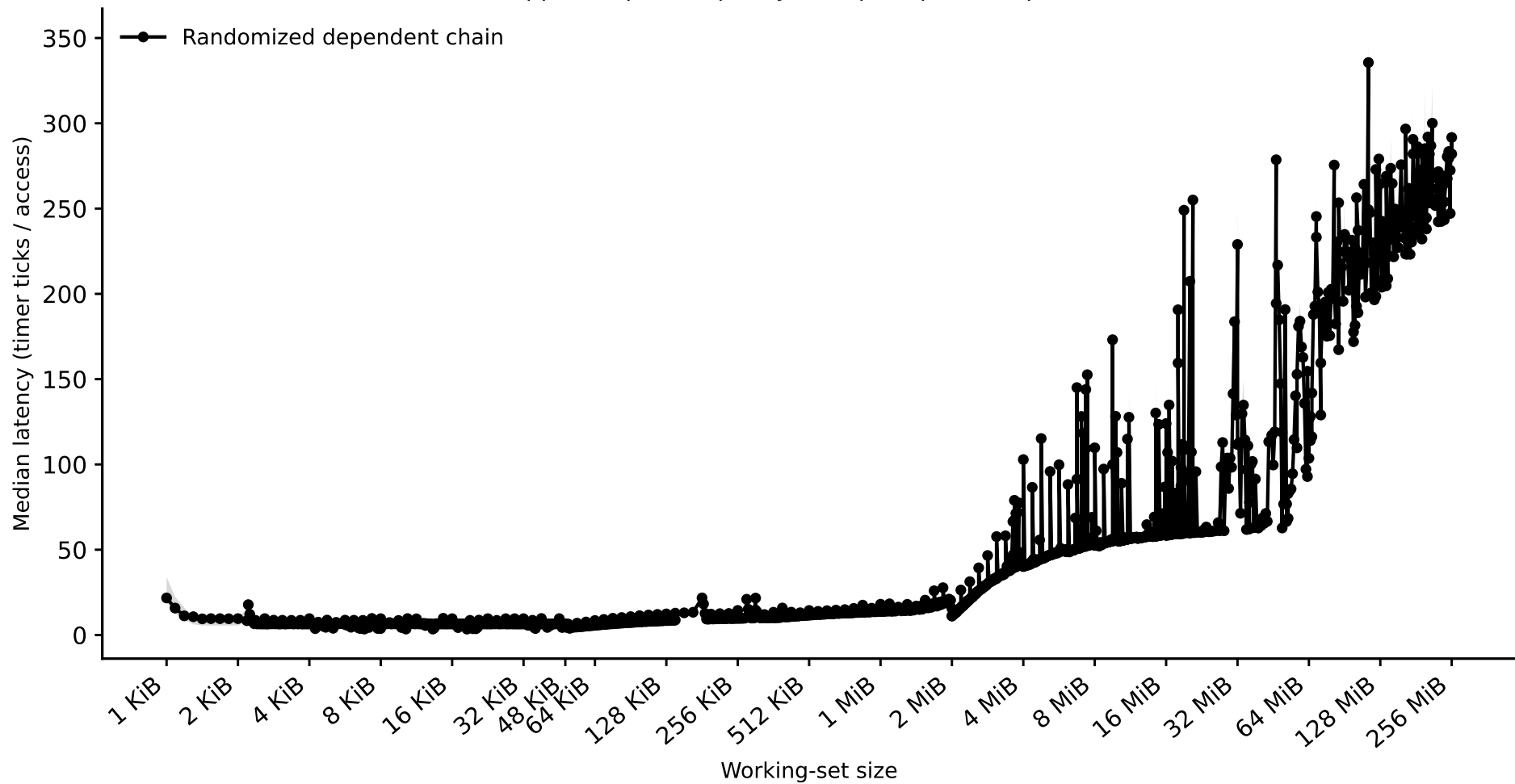
Hazel-Sapphirerapids: capacity sweep (dependent pointer chase)
