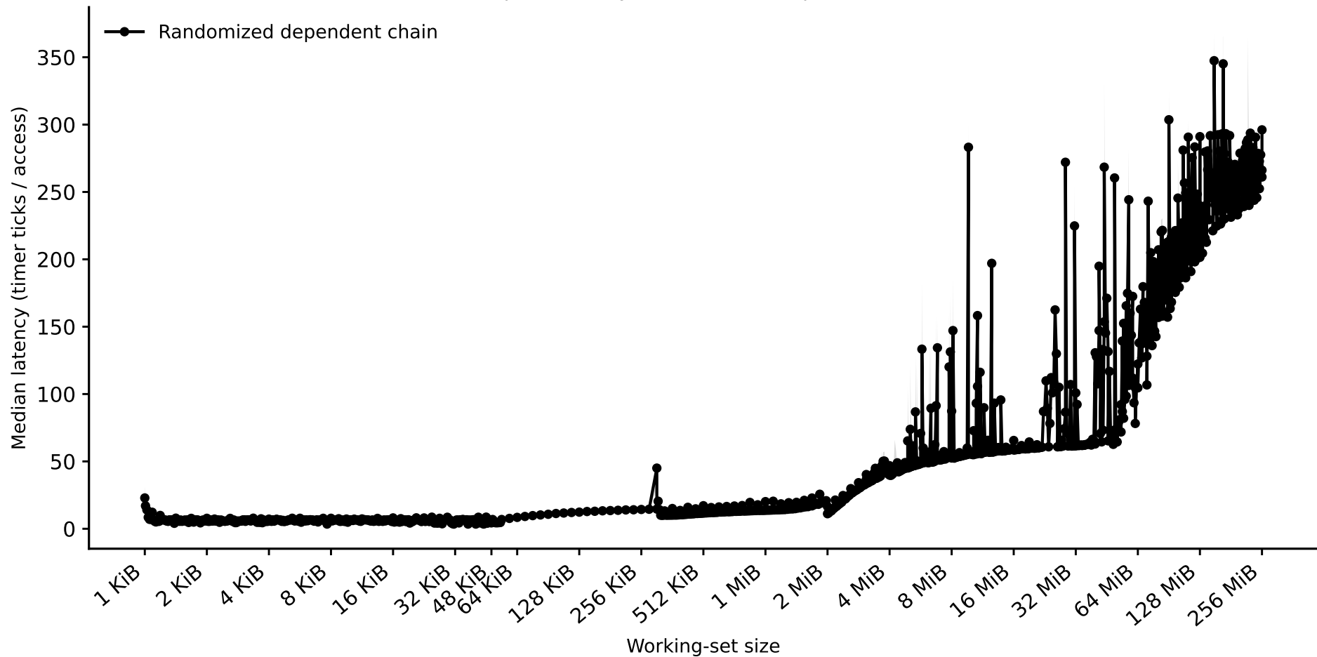
Hazel-Sapphirerapids: capacity sweep (dependent pointer chase) (2026-09-15 reproducibility re-run -- uninterpreted, see CLAUDE.md)
