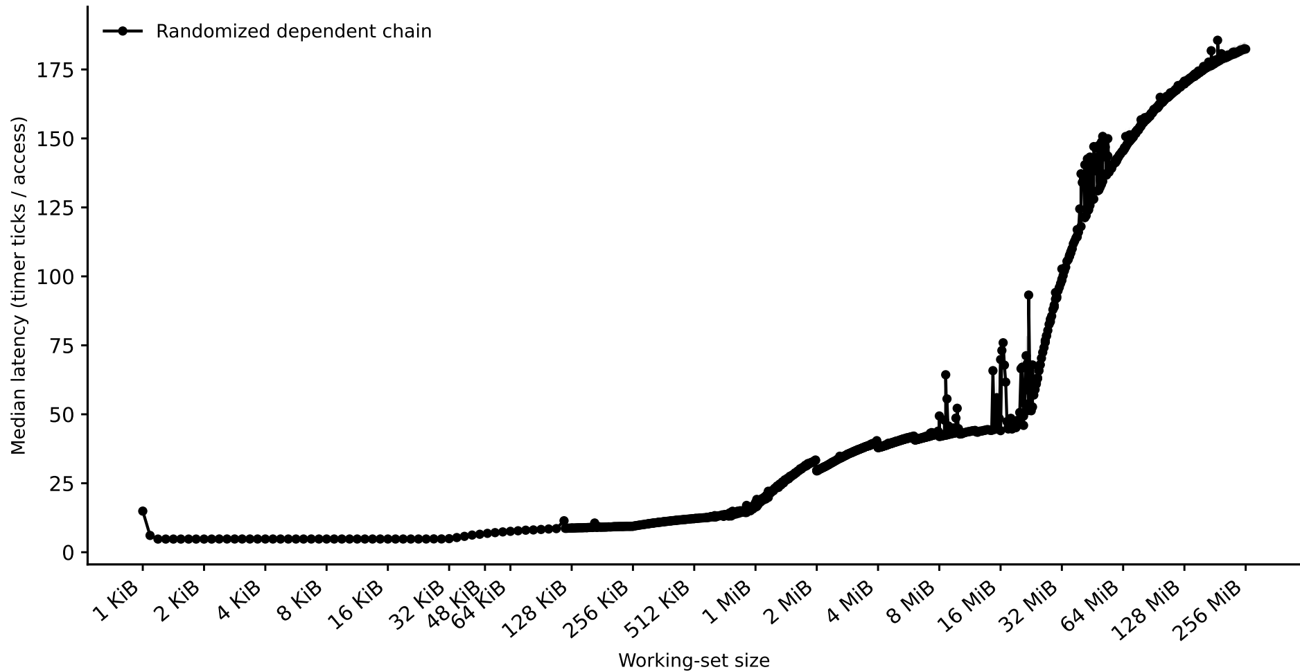
Hazel-Skylake: capacity sweep (dependent pointer chase)
