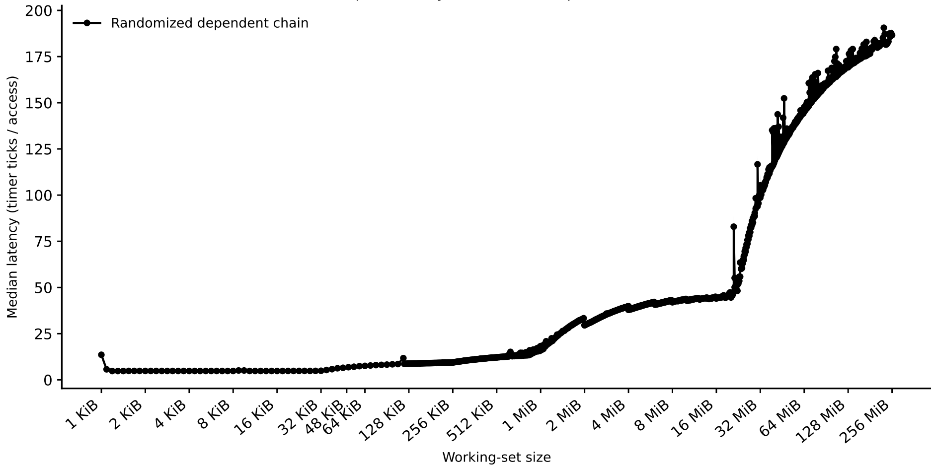
Hazel-Skylake: capacity sweep (dependent pointer chase) (2026-09-15 reproducibility re-run -- uninterpreted, see CLAUDE.md)
