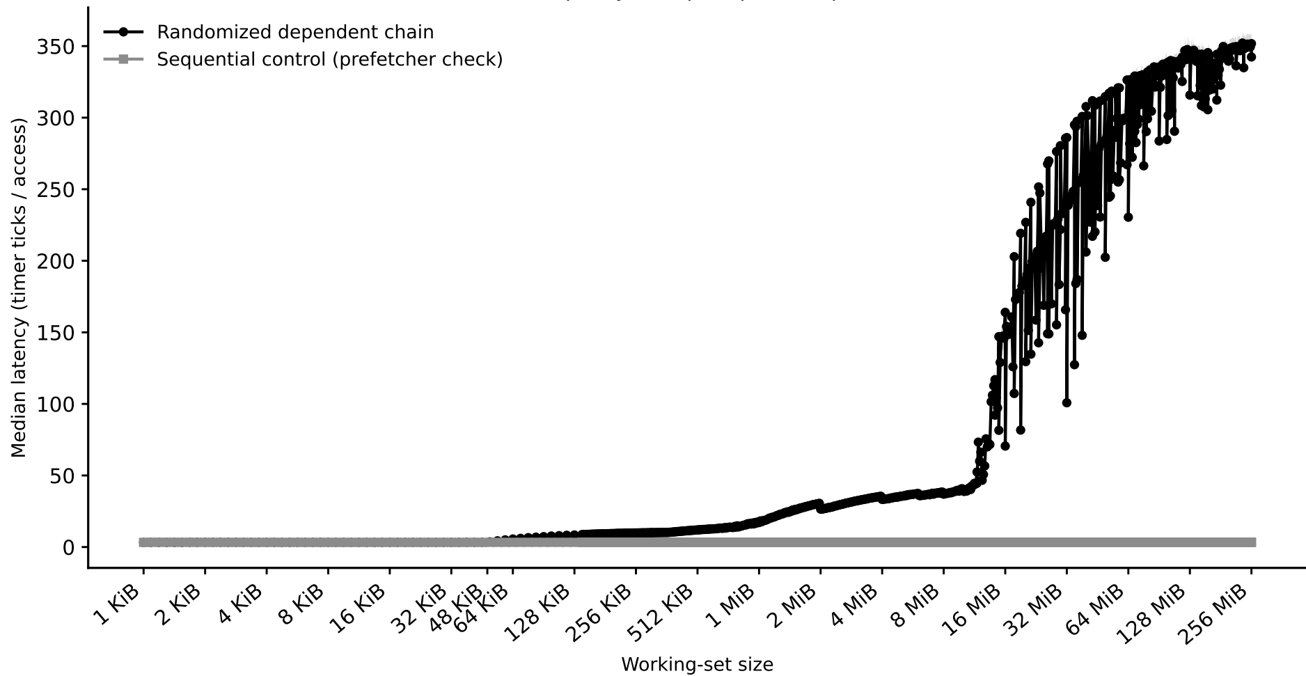
Hazel-Turin: capacity sweep (dependent pointer chase)
