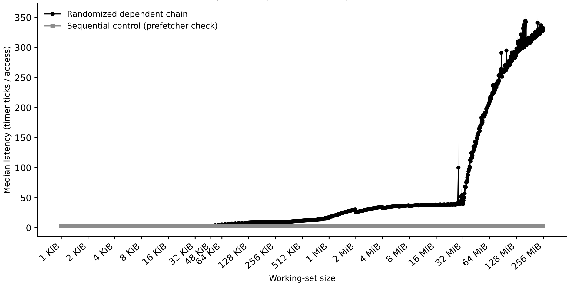
Hazel-Turin: capacity sweep (dependent pointer chase) (2026-09-15 reproducibility re-run -- uninterpreted, see CLAUDE.md)
