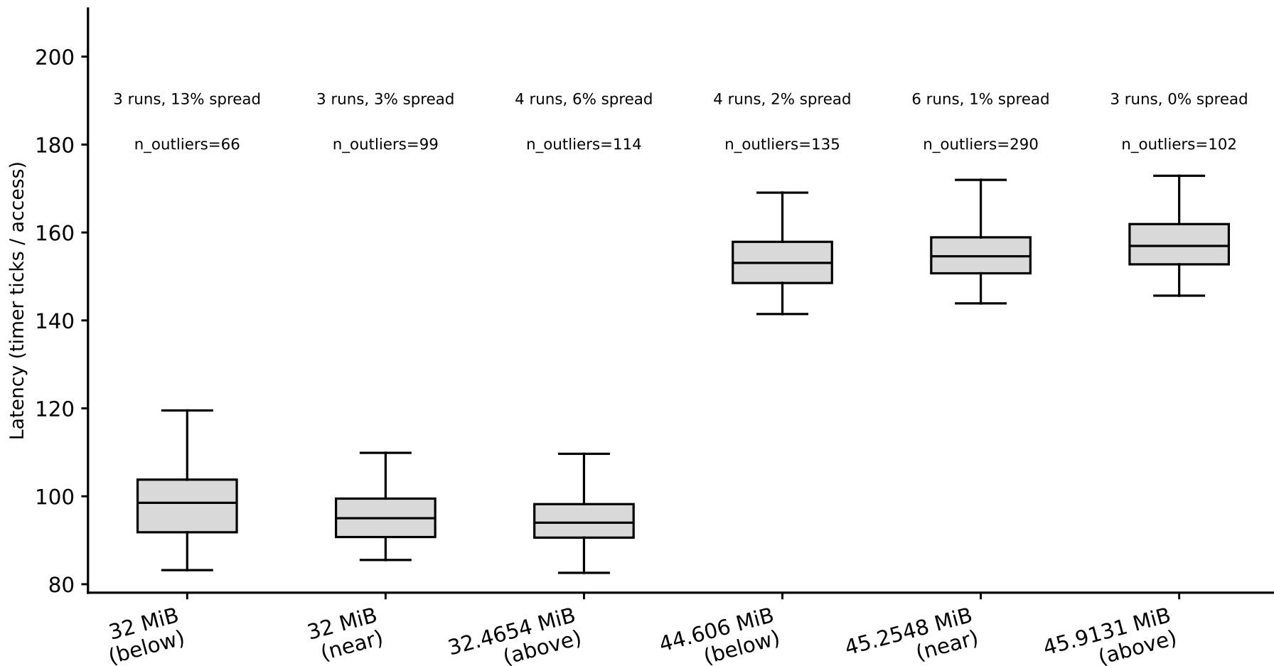
hazel_genoa: capacity box plots, random pattern (whiskers = p5/p95) (Phase I timing-only, auto pipeline) tested boundaries: 32 MiB, 45.2548 MiB
