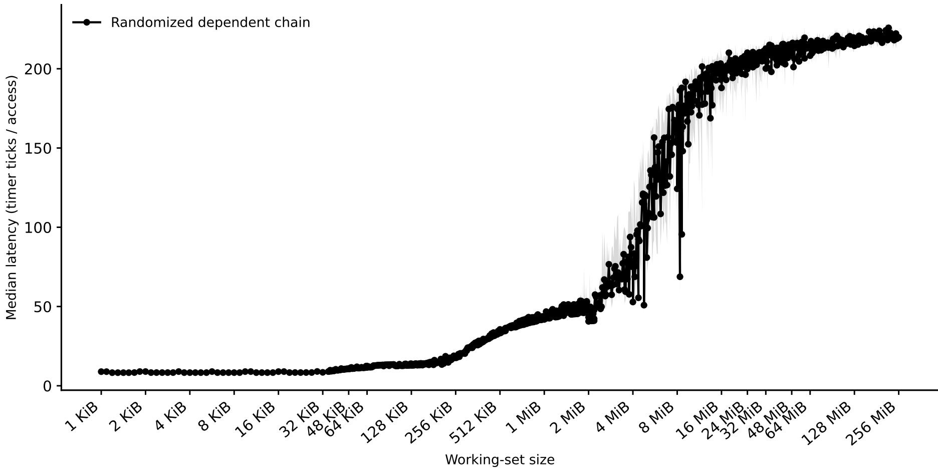
hazel_haswell/capacity_rerun: capacity sweep (dependent pointer chase) (Phase I timing-only, auto pipeline)
