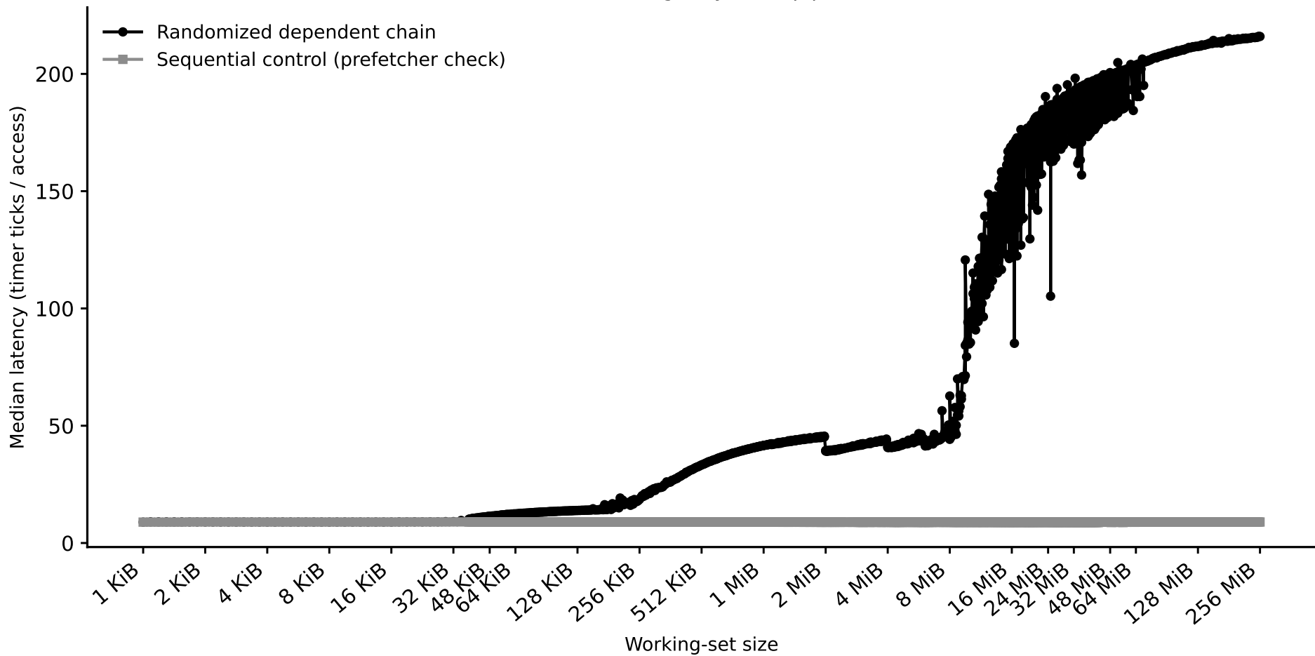
hazel_haswell/capacity_rerun2: capacity sweep (dependent pointer chase) (Phase I timing-only, auto pipeline)
