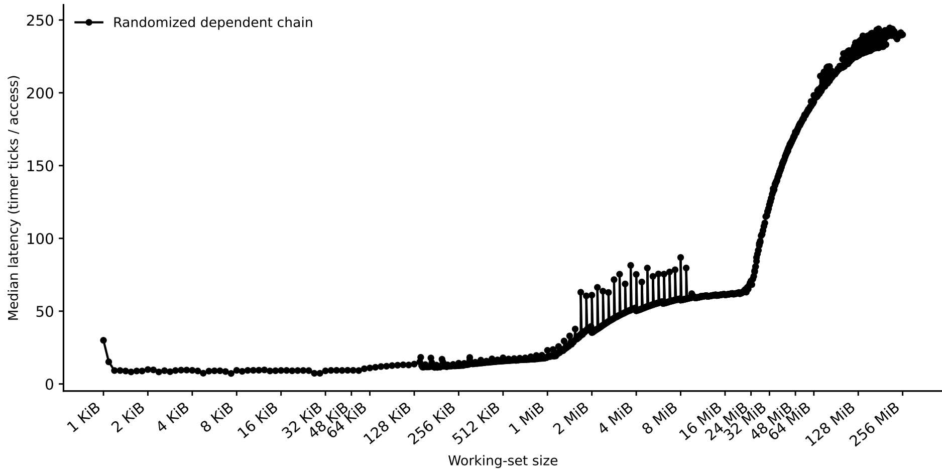
hazel_icelake_6326: capacity sweep (dependent pointer chase) (Phase I timing-only, auto pipeline)
